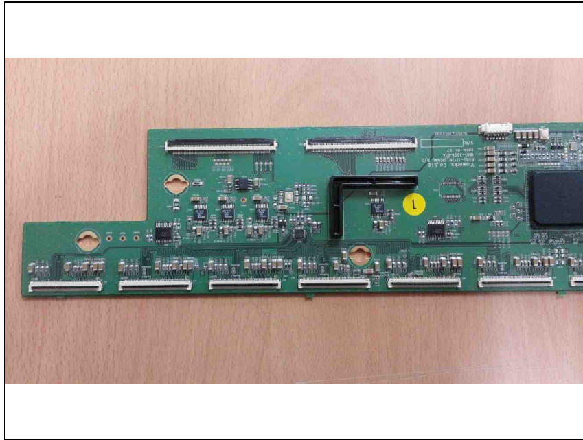
Signal Board_Zoom 1(Top)
