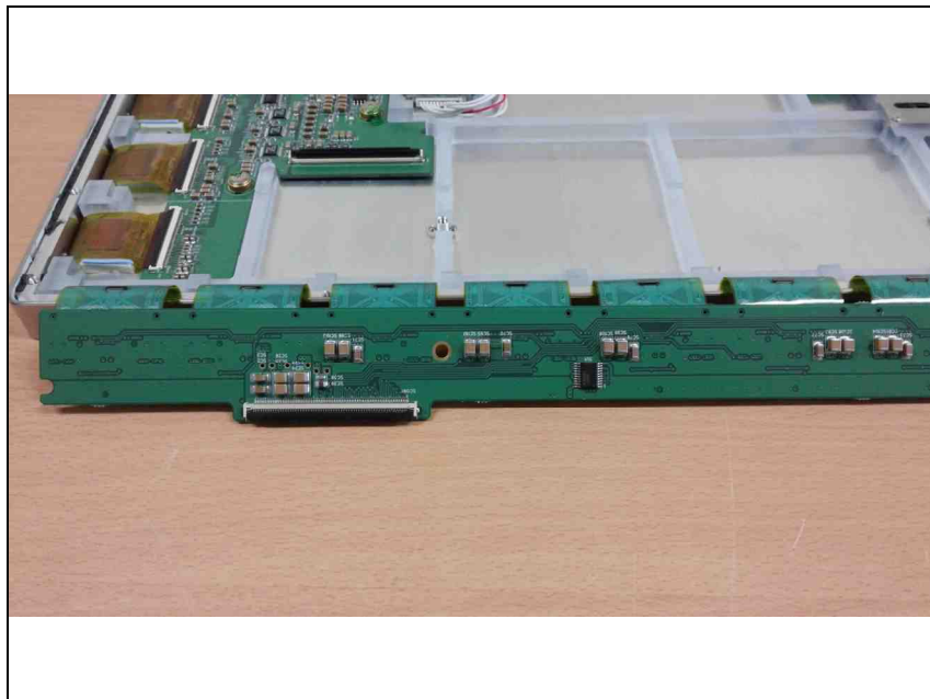
Gate Board_Zoom 1(Bottom)
