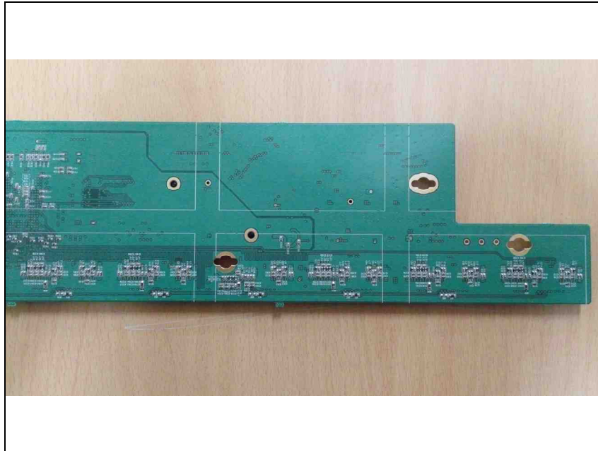
Signal Board_Zoom 2(Bottom)
