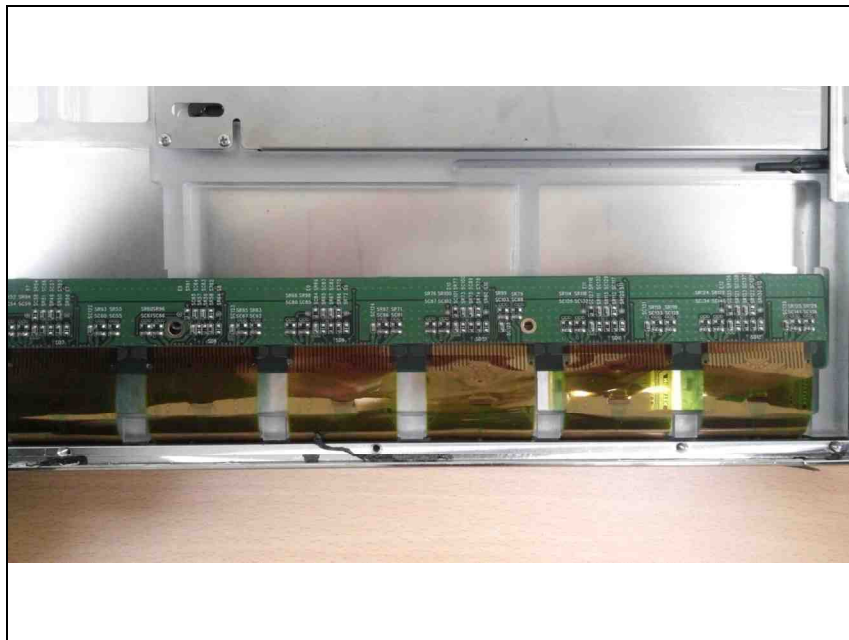
Gate Board_Zoom 2(Top)
