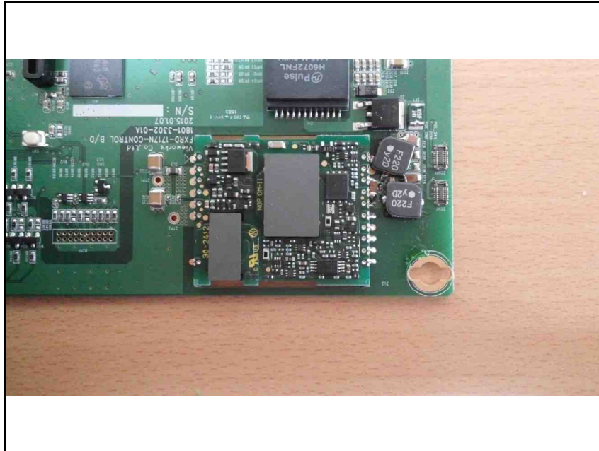
CC30 Board (Shields removed_Top)
