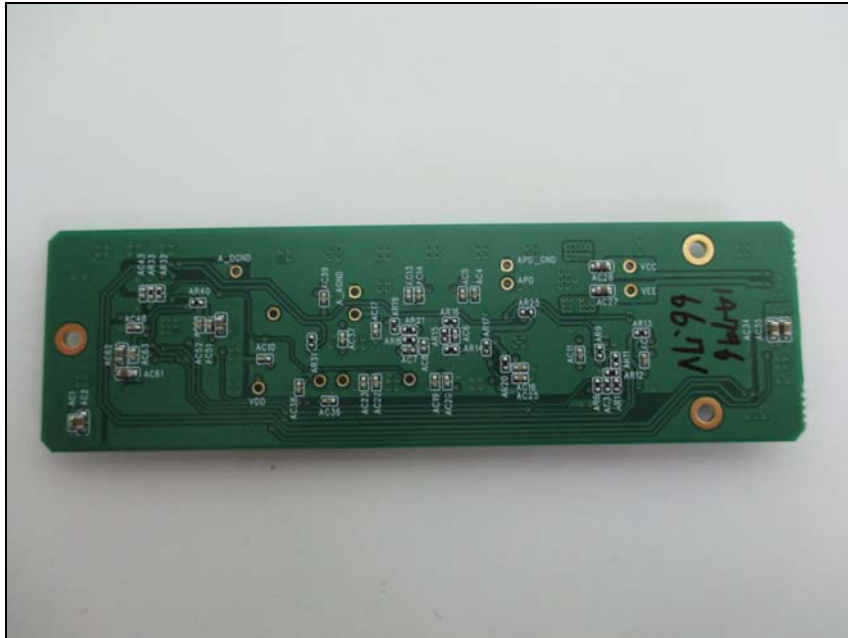
AED board(Bottom)
