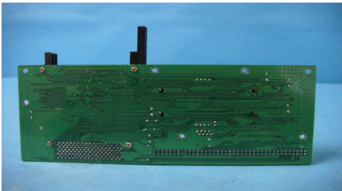
SUB Board PCB Copper View
