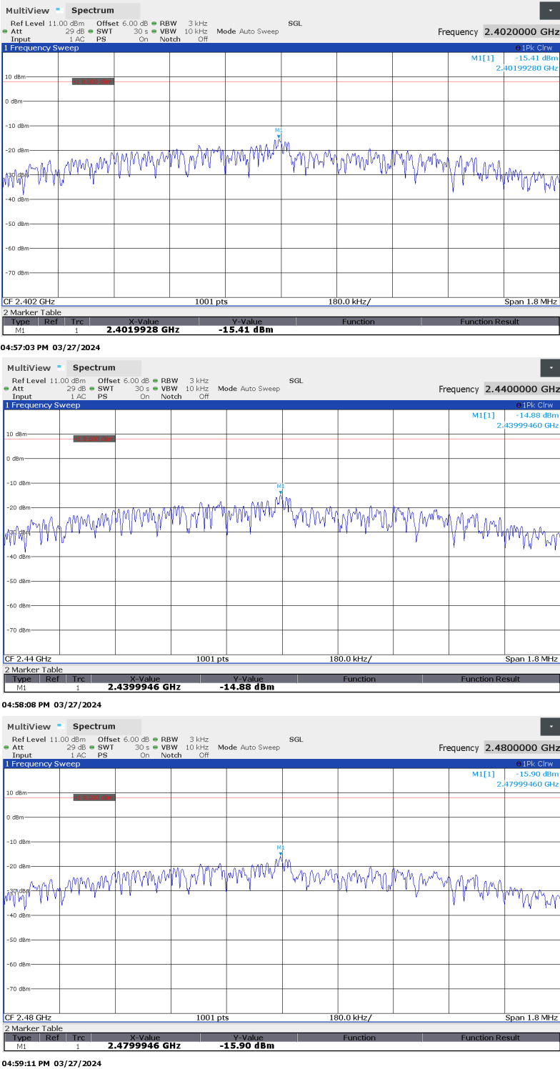
Figure 4.2.4 (ii) Power Spectral Density Plots.
