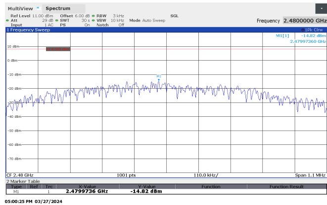
Figure 4.2.4 (i) Power Spectral Density Plots.
