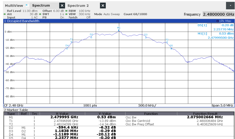
Figure 4.2.2 (ii) Example Intentional Emission Bandwidth Plots.
