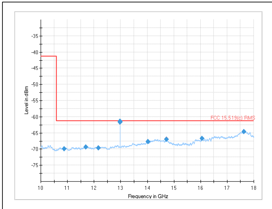
Plot 23: 10 GHz to 18 GHz, UWB test mode channel 5 (SW version 02.11.13)
