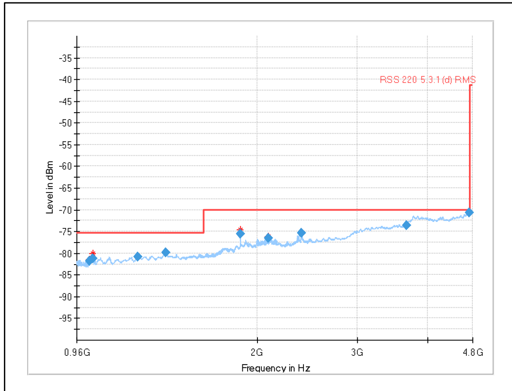
Plot 16: 960 MHz to 4.8 GHz (Limit acc. to RSS-220 5.3.1(d)), UWB test mode channel 5 (SW version 02.11.13)
