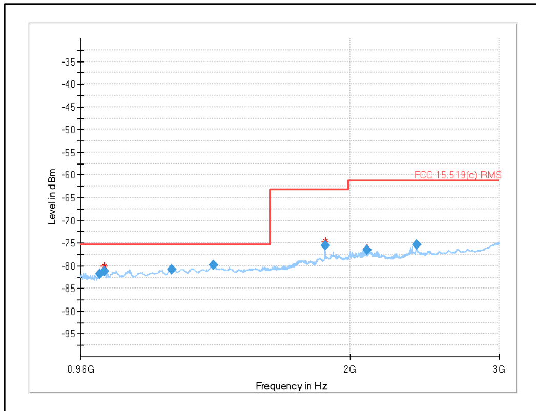
Plot 15: 960 MHz to 3 GHz (Limit acc. to §15.519 (c)), UWB test mode channel 5 (SW version 02.11.13)
