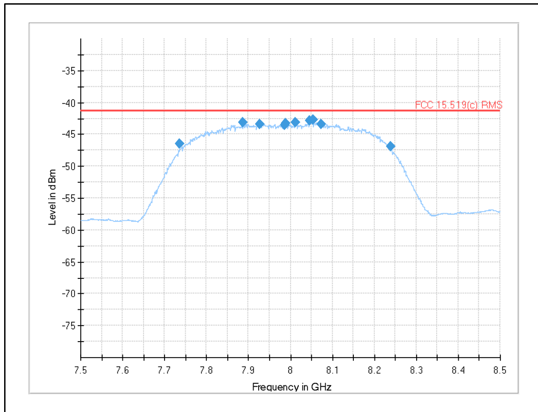
Plot 7: Fundamental emission (UWB test mode): RMS channel 9 (SW version 02.11.13)
