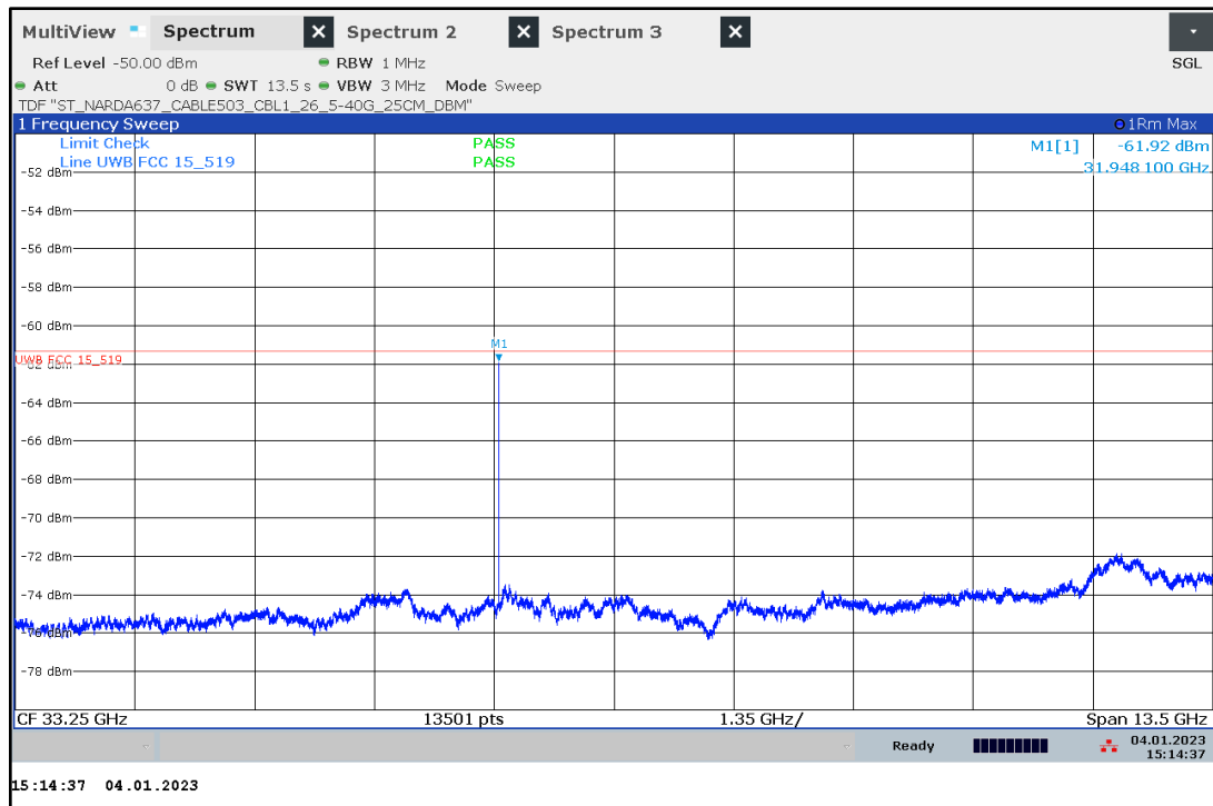
Plot 33: 26.5 GHz to 40.0 GHz, UWB test mode channel 9, prescan (SW version 02.11.13)
