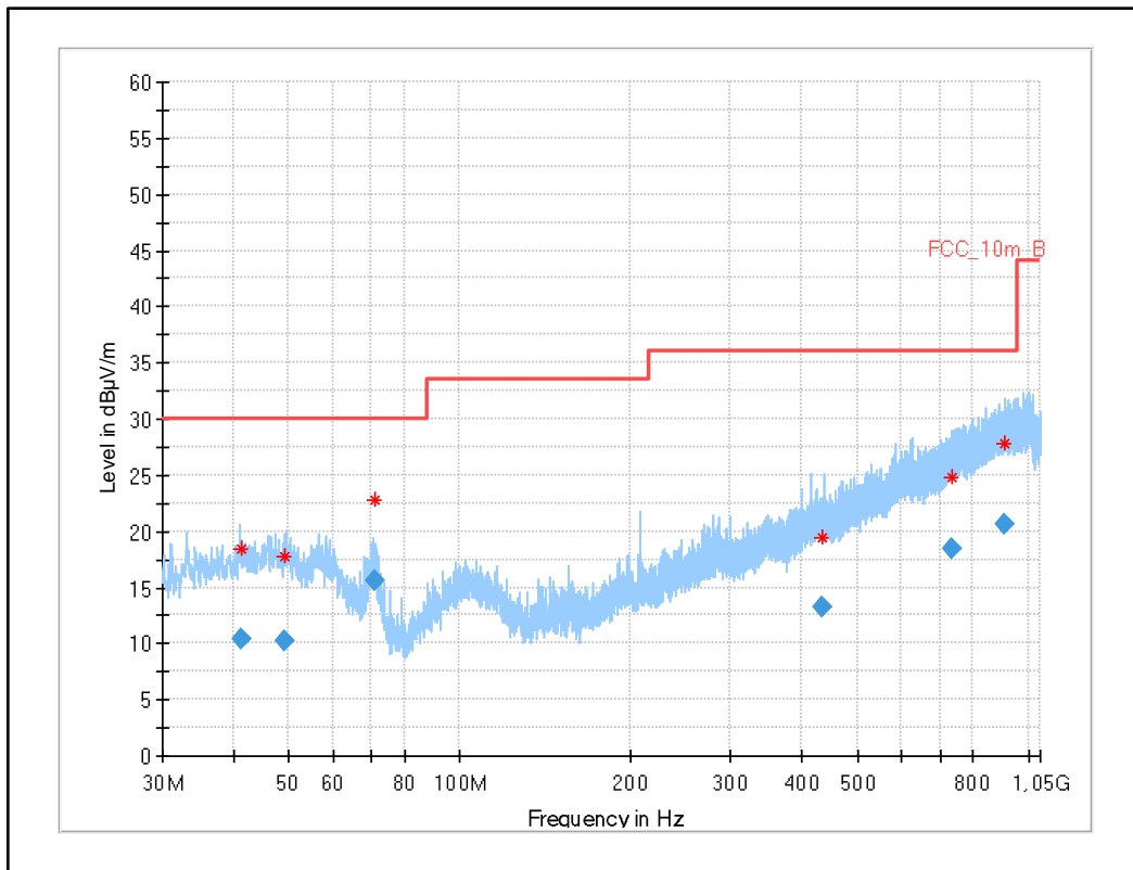
Plot 14: 30 MHz to 1 GHz, UWB test mode channel 9 (SW version 02.11.13)
