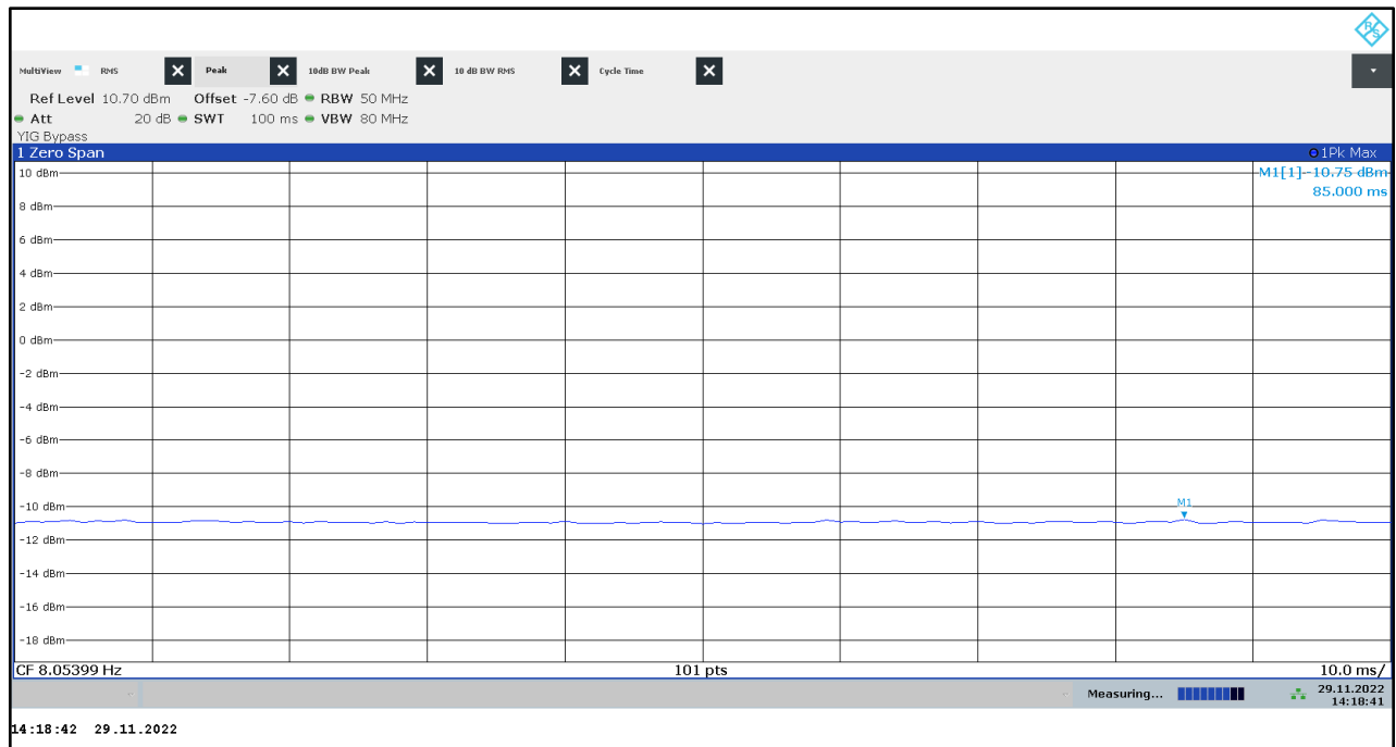
Plot 9: Fundamental emission (UWB test mode): Max Peak channel 9 (SW version 02.11.13)
