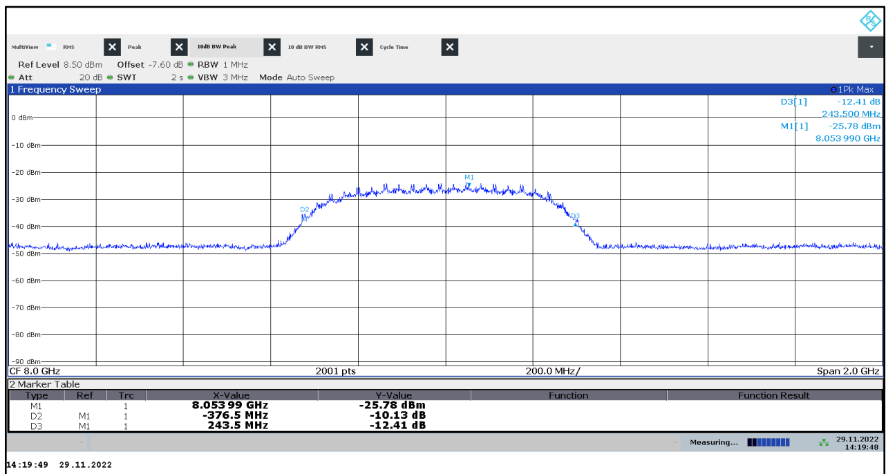
Plot 2: 10 dB bandwidth, UWB test mode channel 9 (SW version 02.11.13)
