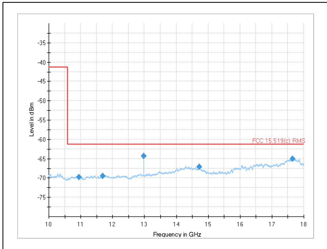
Plot 24: 10 GHz to 18 GHz, UWB test mode channel 5 (SW version 02.12.13)
