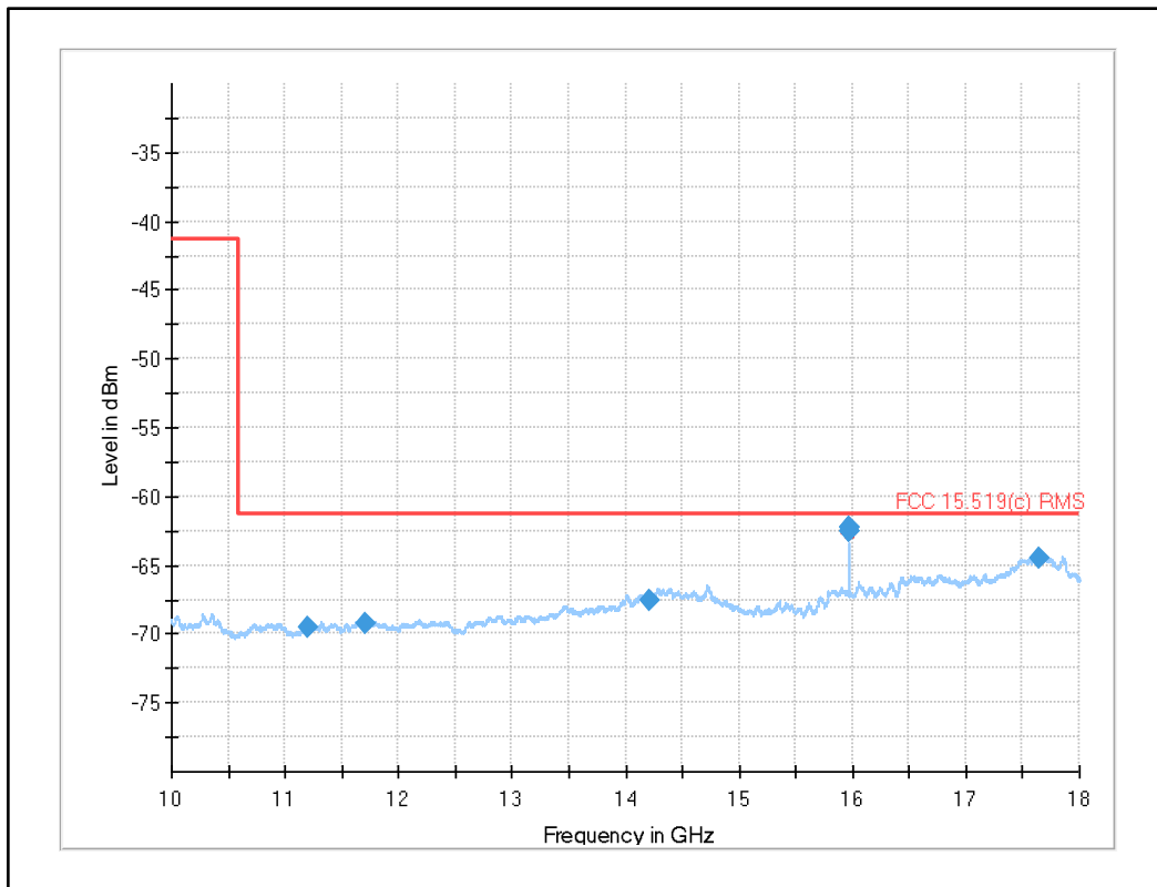
Plot 25: 10 GHz to 18 GHz, UWB test mode channel 9 (SW version 02.11.13)
