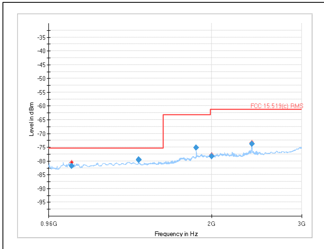
Plot 17: 960 MHz to 3 GHz (Limit acc. to §15.519 (c)), UWB test mode channel 9 (SW version 02.11.13)
