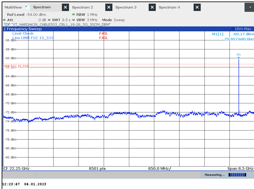
Plot 27: 18 GHz to 26.5 GHz, UWB test mode channel 5, prescan (SW version 02.11.13)
