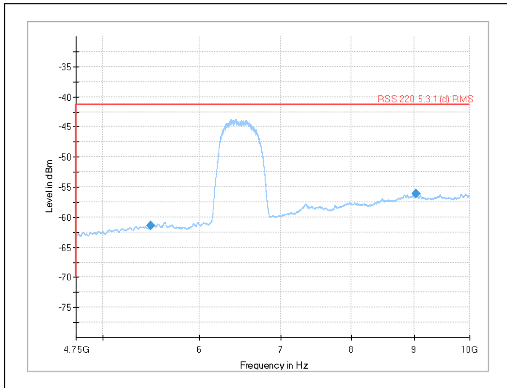
Plot 20: 4.75 GHz to 10 GHz, UWB test mode channel 5 (SW version 02.11.13)
