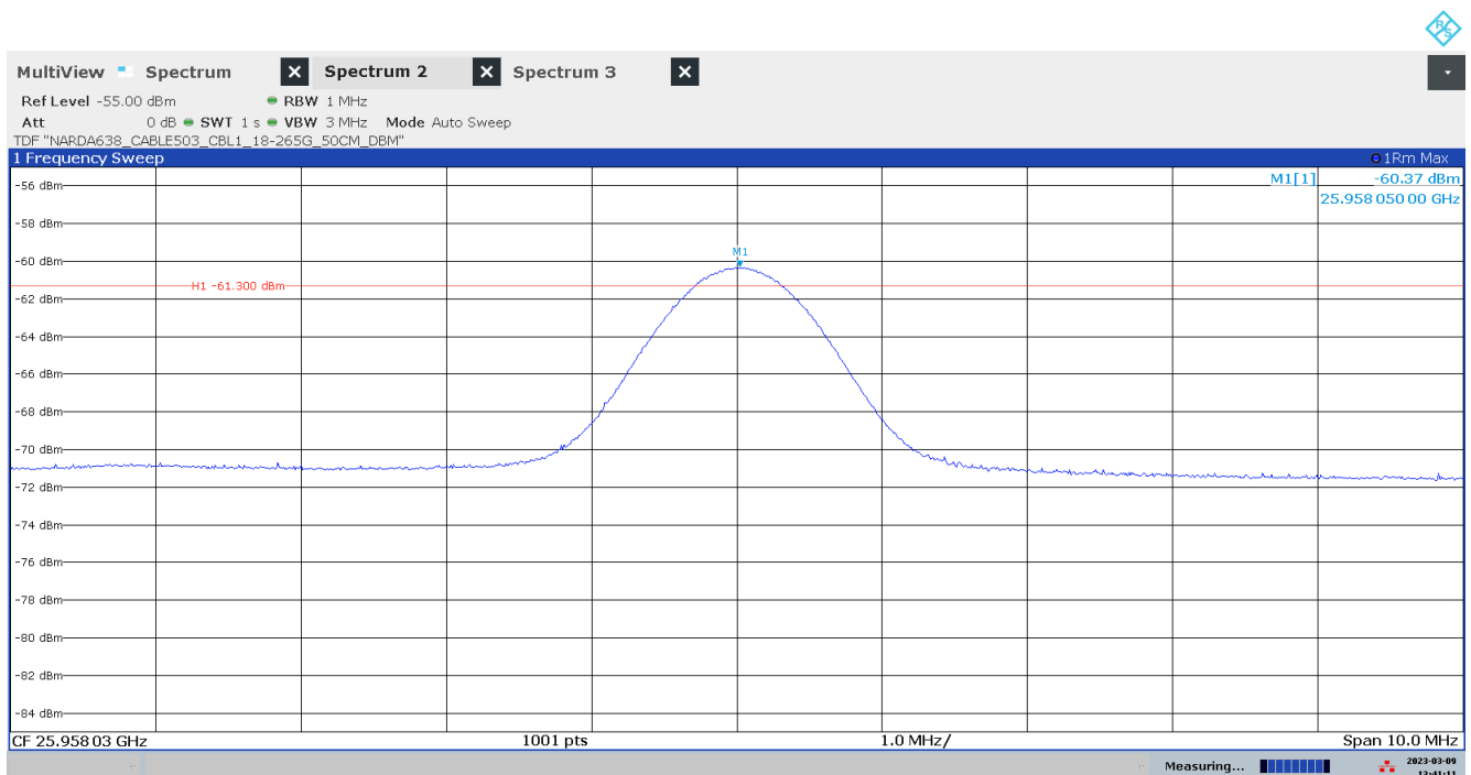
Plot 28: Detailed measurement, f_c = 25.958 GHz, UWB test mode channel 5 (SW version 02.12.13)
