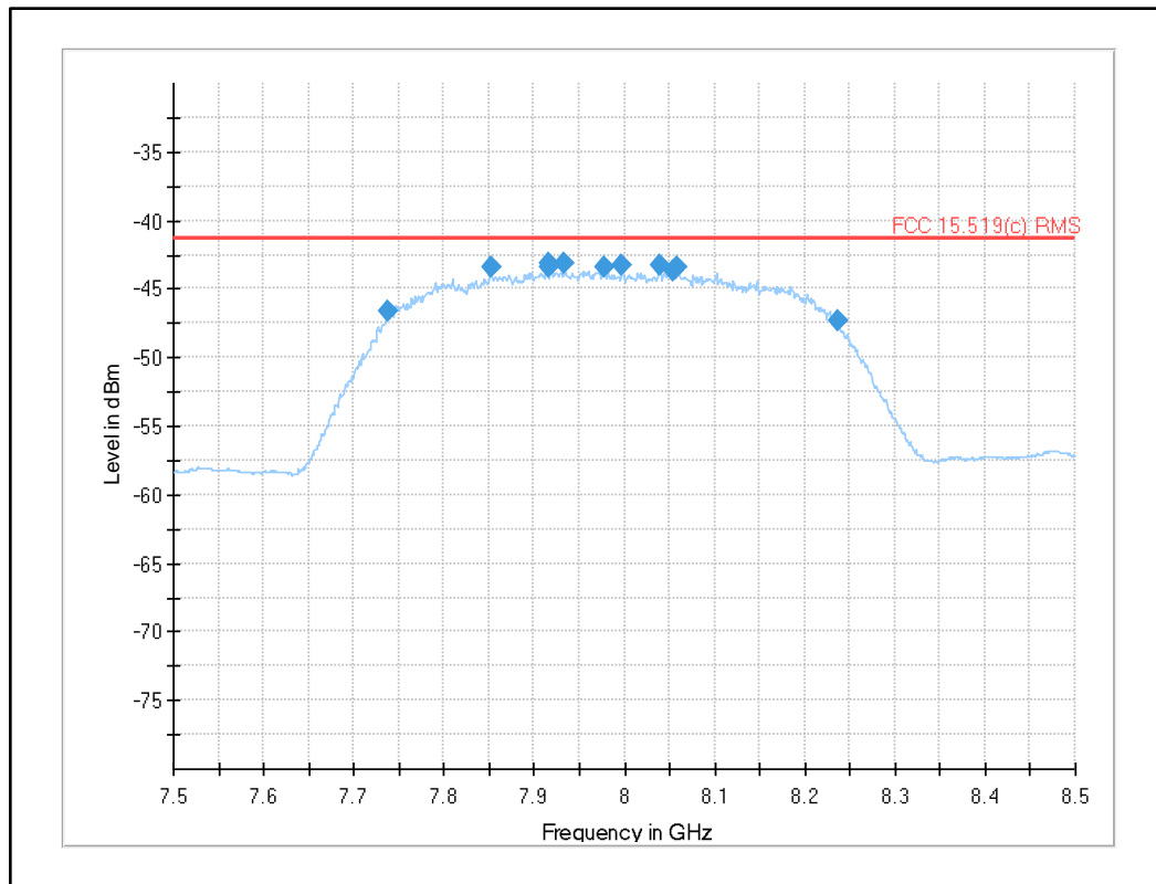
Plot 8: Fundamental emission (UWB test mode): RMS channel 9 (SW version 02.12.13)
