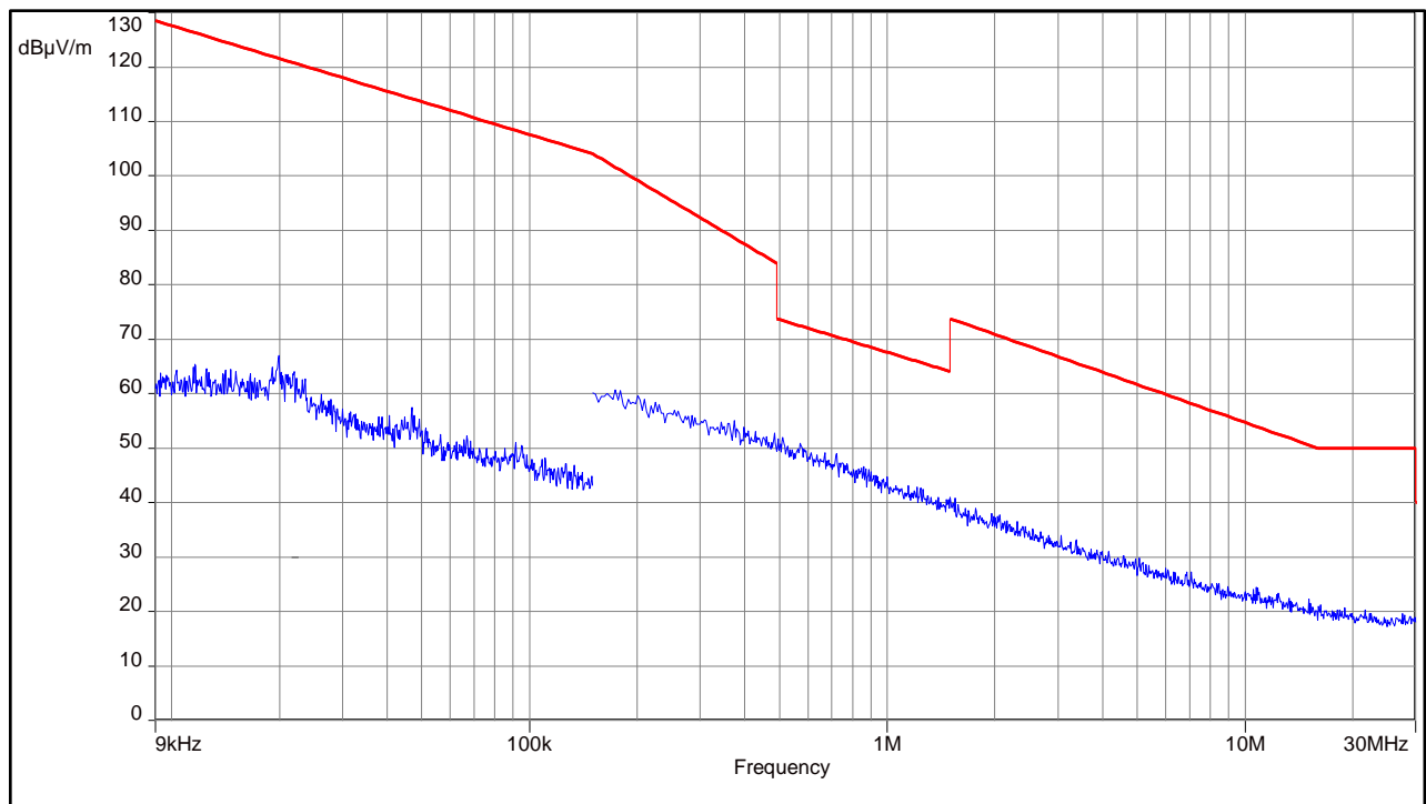
Plot 12: 9 kHz to 30 MHz, UWB test mode channel 9 (SW version 02.11.13)
