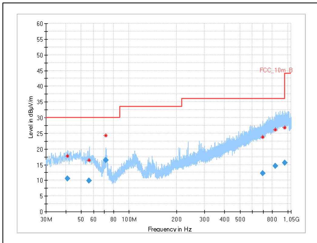
Plot 13: 30 MHz to 1 GHz, UWB test mode channel 5 (SW version 02.11.13)
