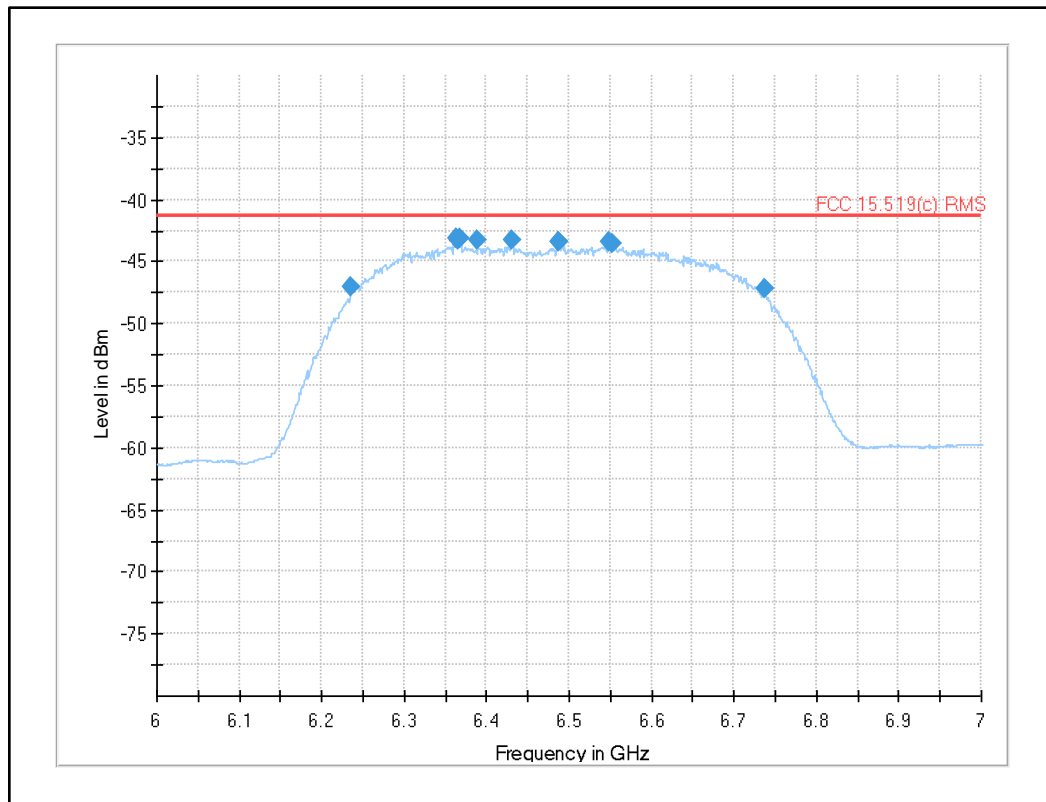
Plot 3: Fundamental emission (UWB test mode): RMS channel 5 (SW version 02.11.13)
