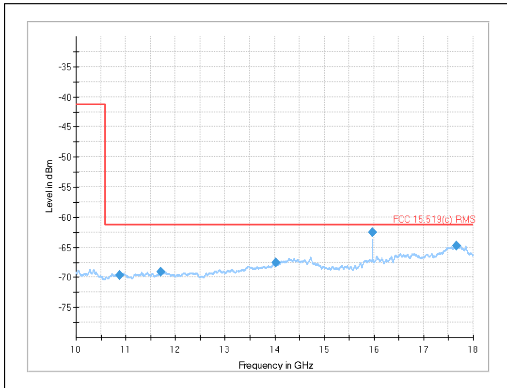
Plot 26: 10 GHz to 18 GHz, UWB test mode channel 9 (SW version 02.12.13)
