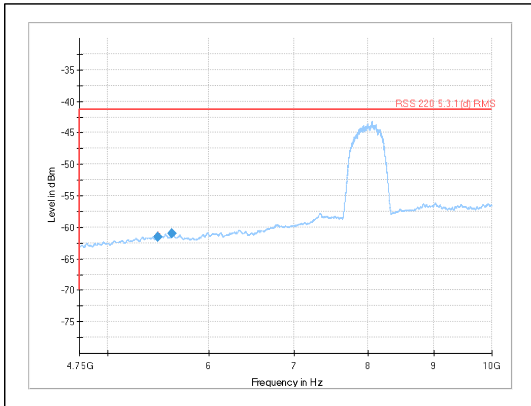
Plot 22: 4.75 GHz to 10 GHz, UWB test mode channel 9 (SW version 02.11.13)
