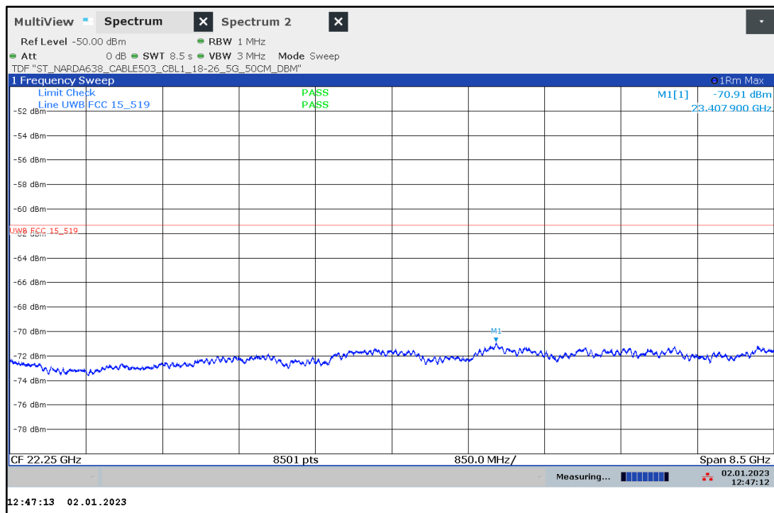
Plot 32: 18 GHz to 26.5 GHz, UWB test mode channel 9 (SW version 02.11.13)
