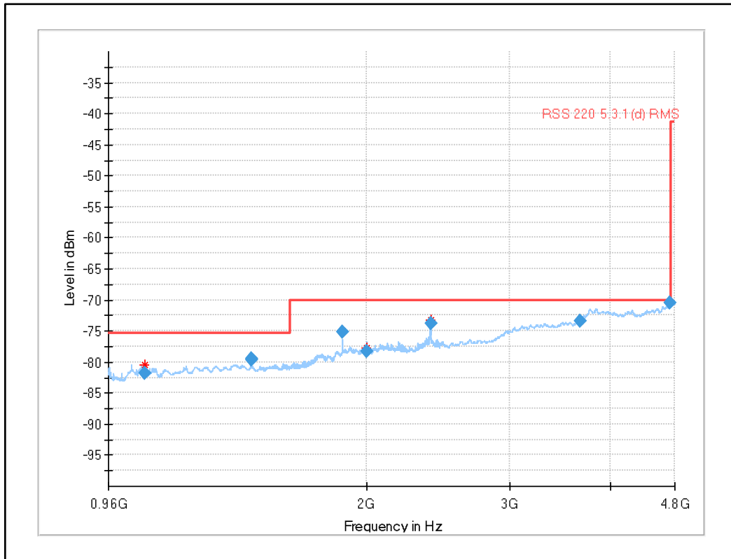
Plot 18: 960 MHz to 4.8 GHz (Limit acc. to RSS-220 5.3.1(d)), UWB test mode channel 9 (SW version 02.11.13)
