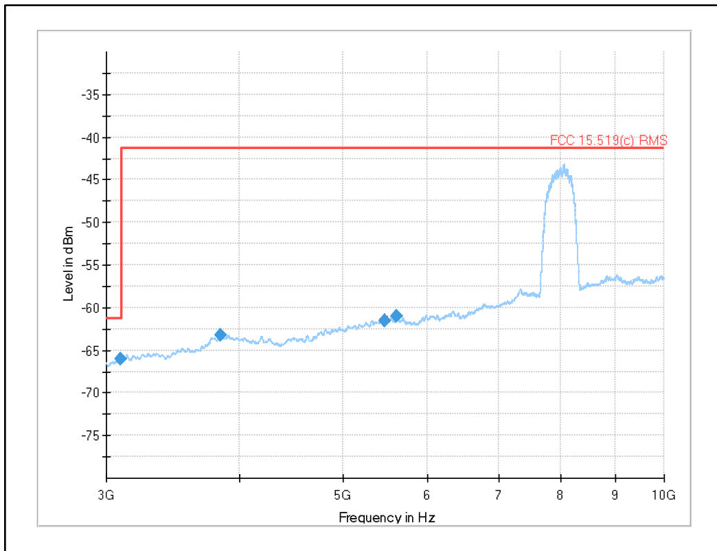
Plot 21: 3 GHz to 10 GHz, UWB test mode channel 9 (SW version 02.11.13)
