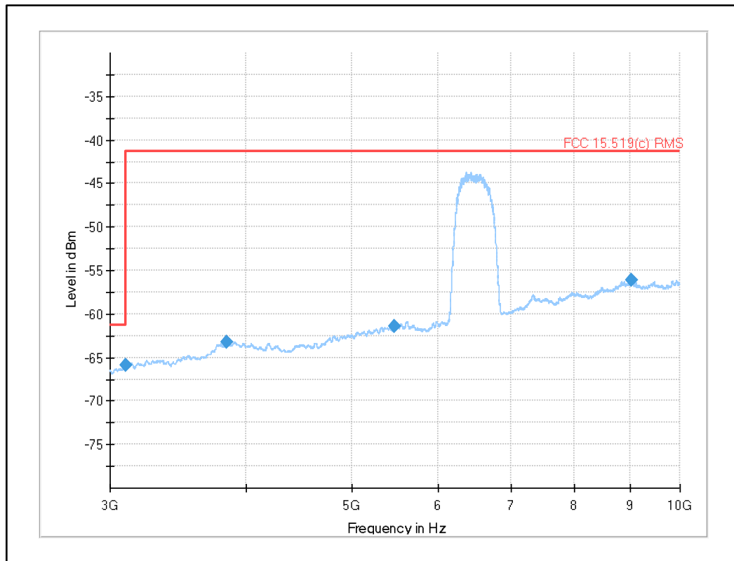
Plot 19: 3 GHz to 10 GHz, UWB test mode channel 5 (SW version 02.11.13)
