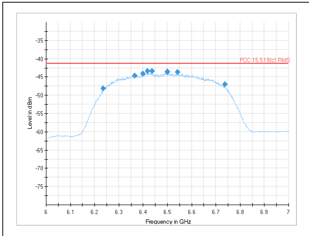
Plot 4: Fundamental emission (UWB test mode): RMS channel 5 (SW version 02.12.13)
