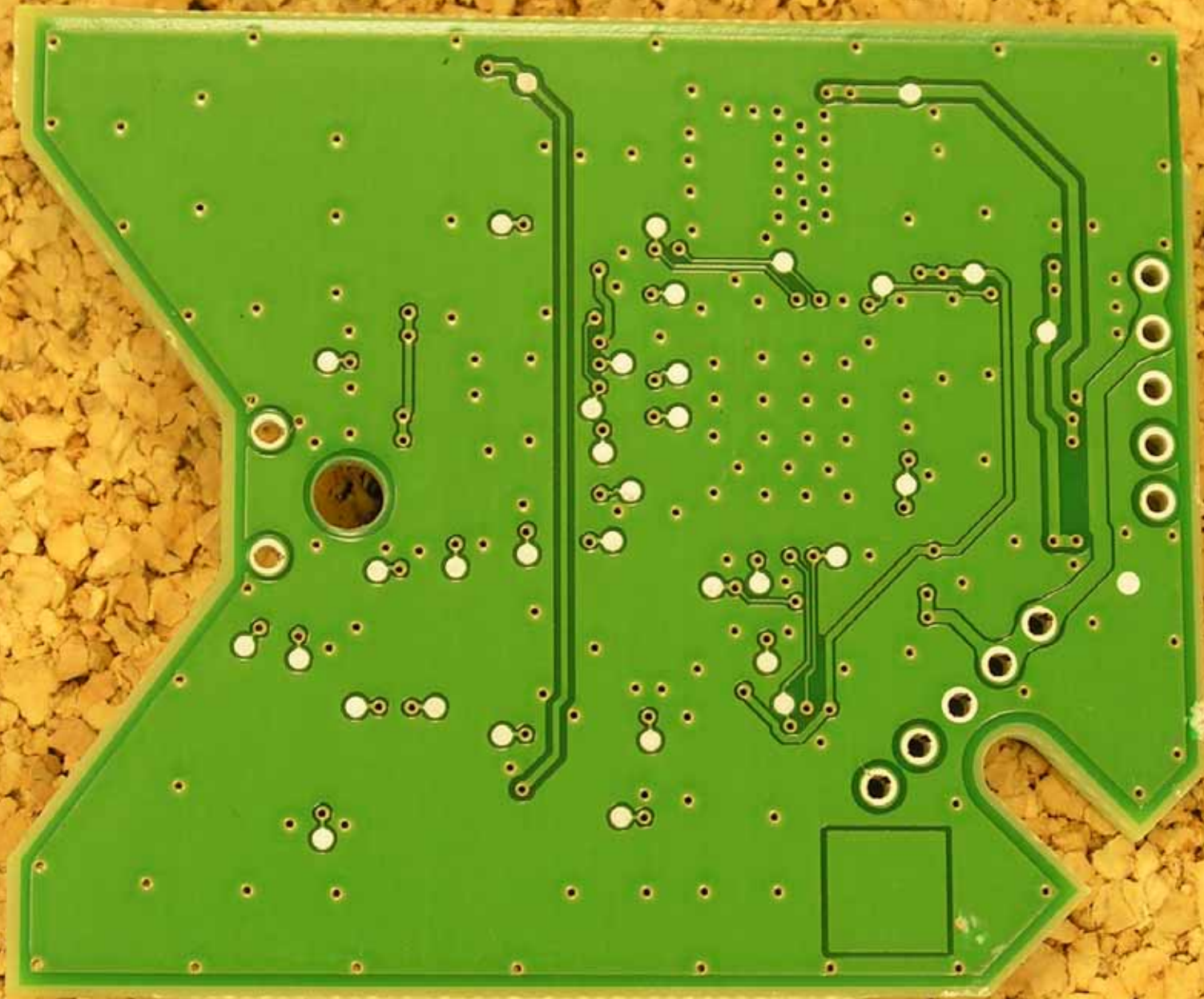
PCB (bottom)
