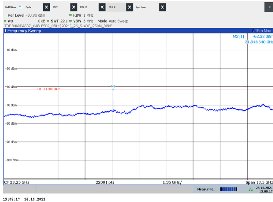
Plot 19: 26 GHz to 40 GHz, CH 9
