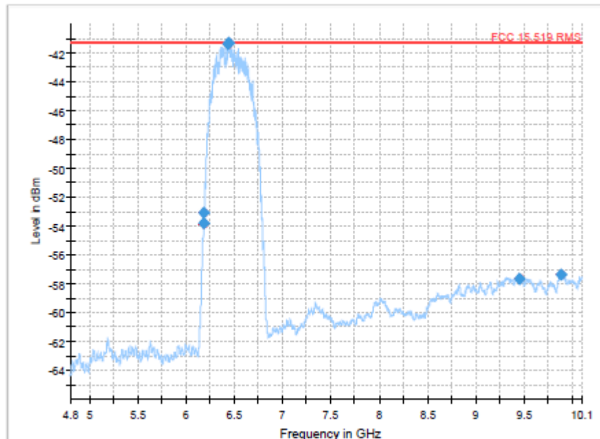
Plot 3: Fundamental emission, CH 5
