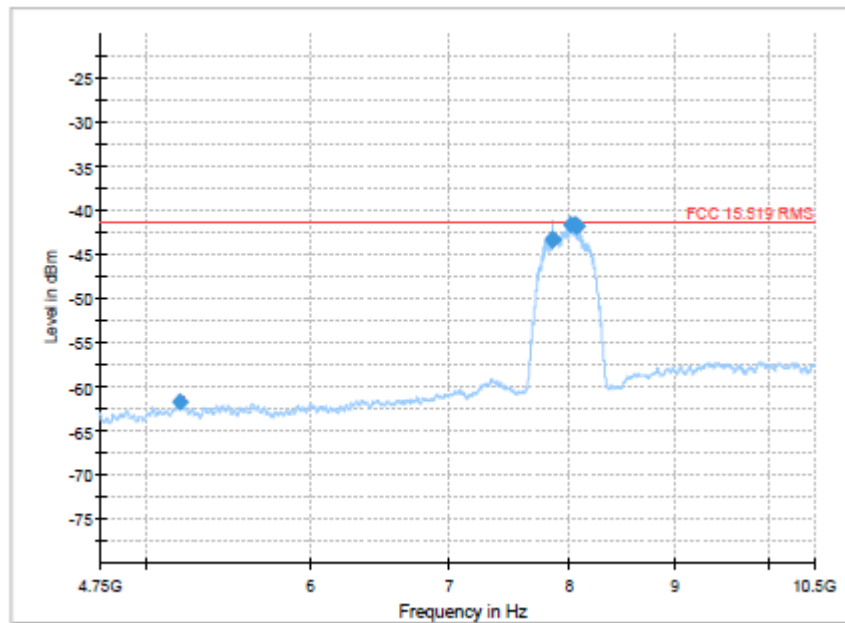
Plot 6: Peak fundamental emission, CH 9
