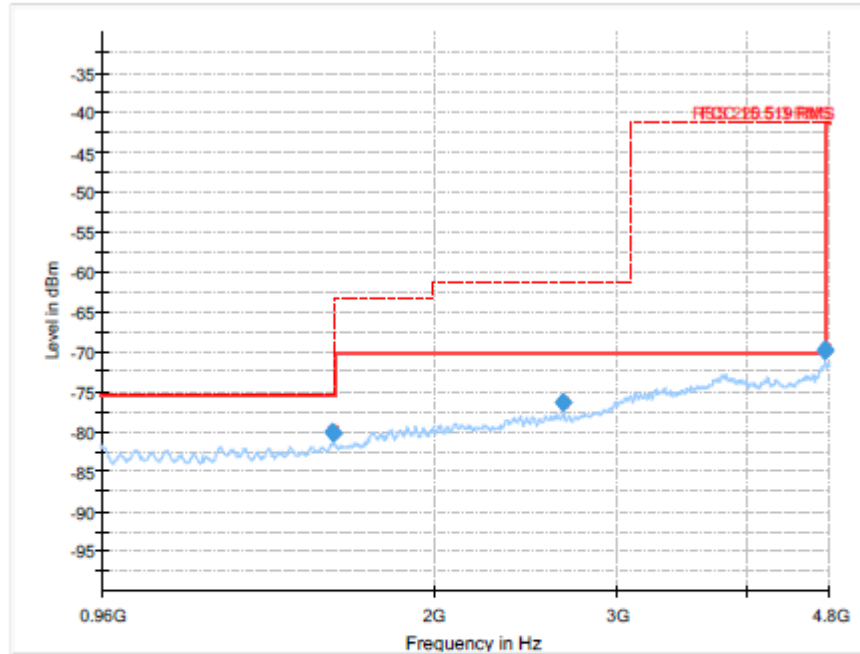
Plot 12: 960 MHz to 4.8 GHz, CH 9
