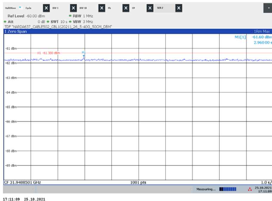
Plot 20: 31949 MHz zoom in, CH 9
