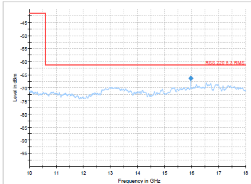
Plot 16: 10 GHz to 18 GHz, CH 9
