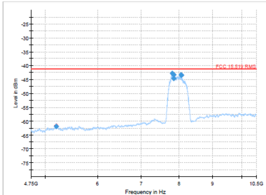
Plot 14: 4.75 GHz to 10.5 GHz, CH 9
