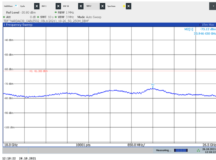
Plot 18: 18 GHz to 26.5 GHz, CH 9
