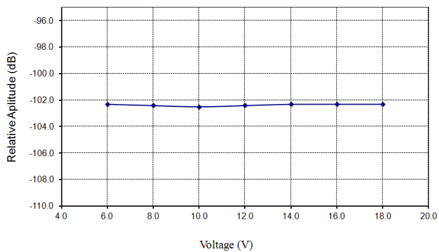
Figure 6.4. Relative emission vs. supply voltage.
