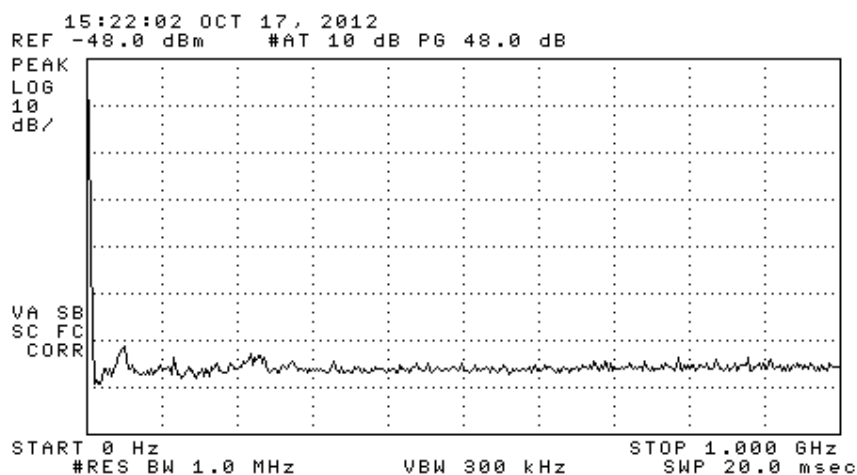
Figure 6.1. Emissions measured at 3 meters in chamber, 0-1000 MHz.
