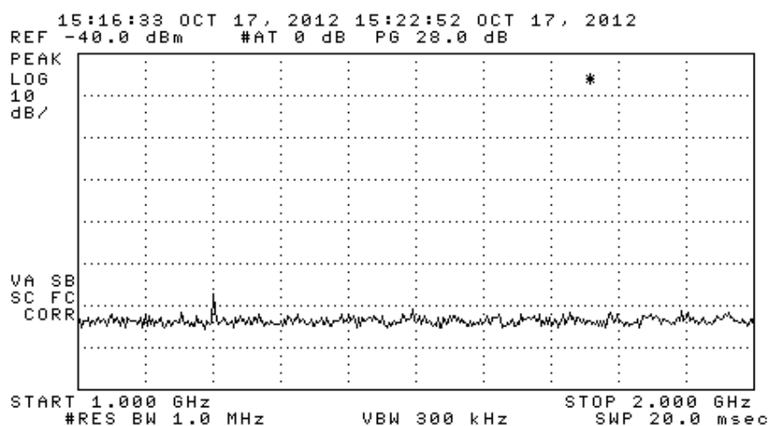
Figure 6.2. Emissions measured at 3 meters in chamber, 1000-2000 MHz. (emission at 1.2 GHz is background)
