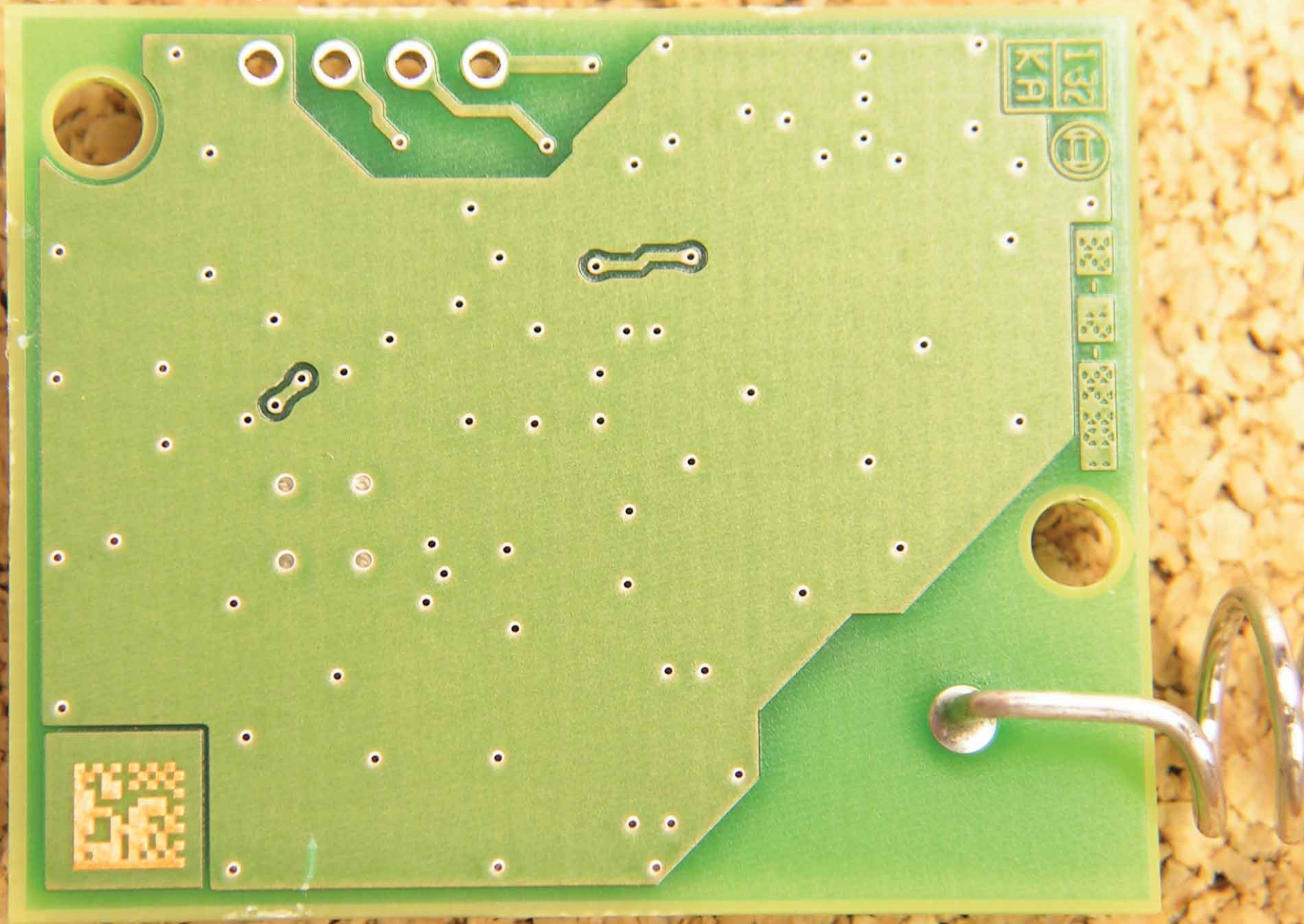
PCB (bottom)
