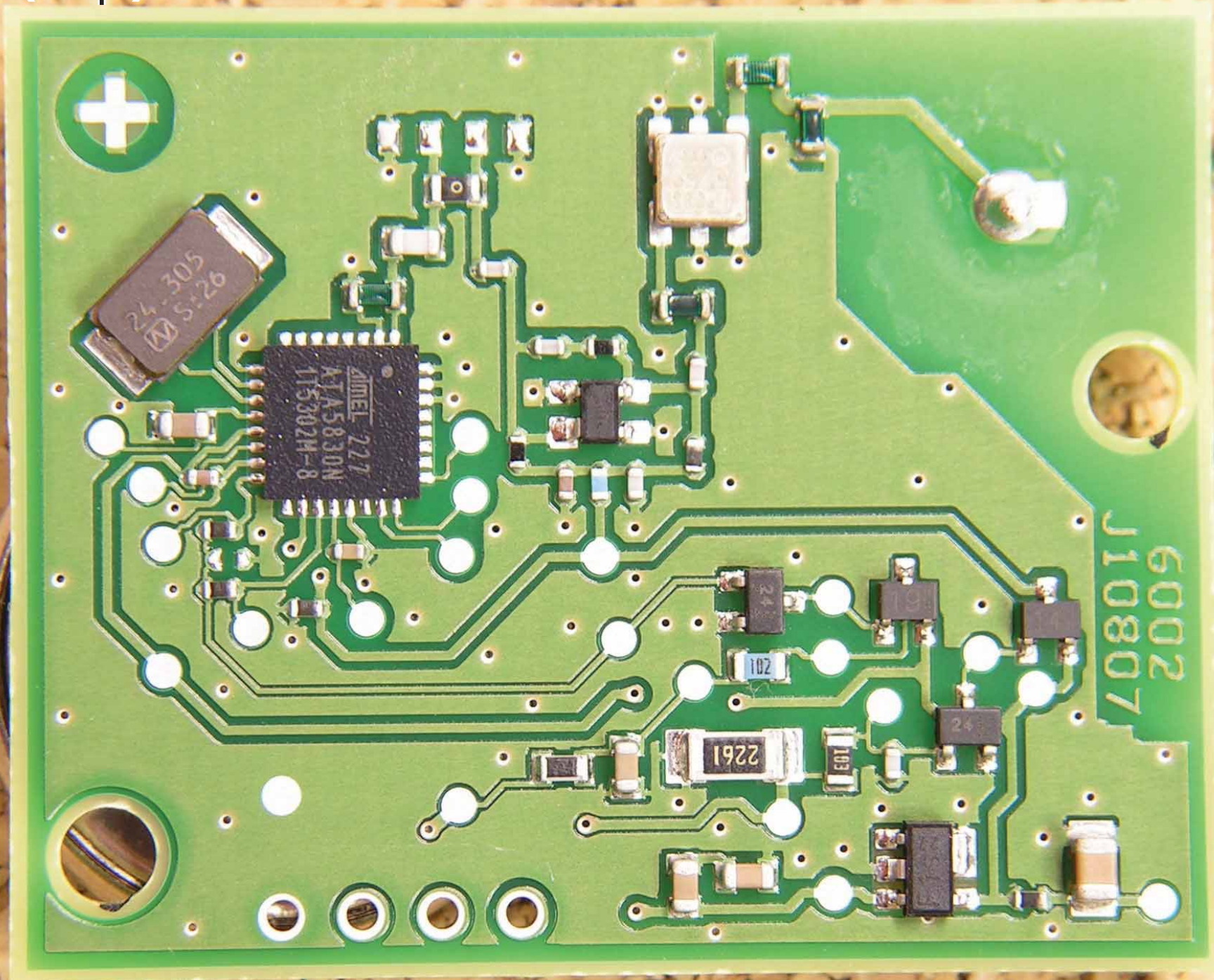
PCB (top)
