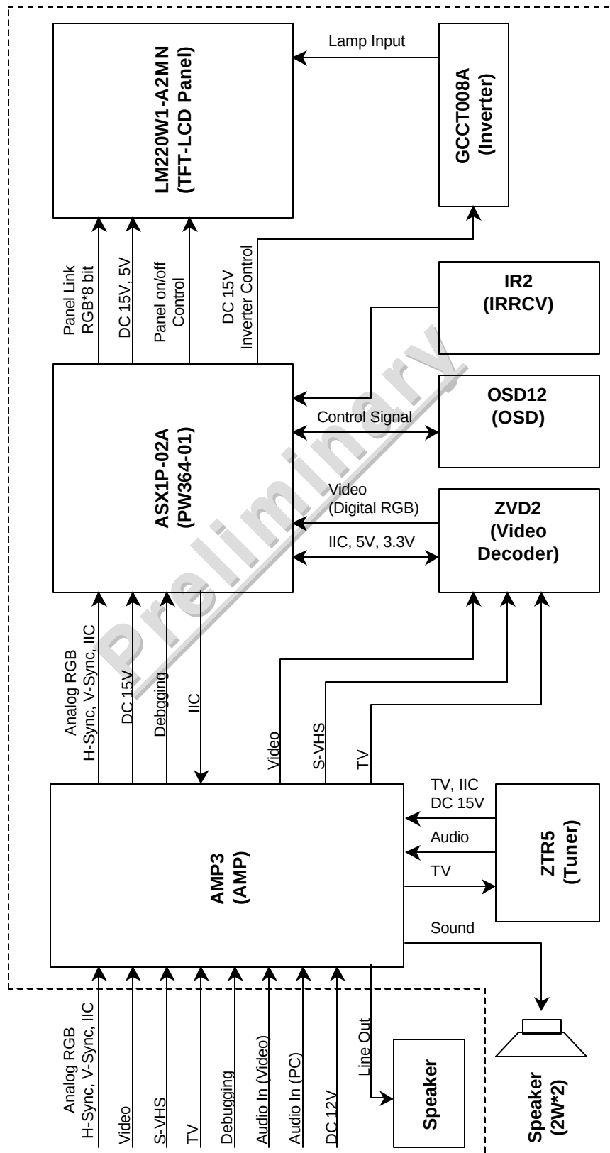
TM800 Block Diagram
