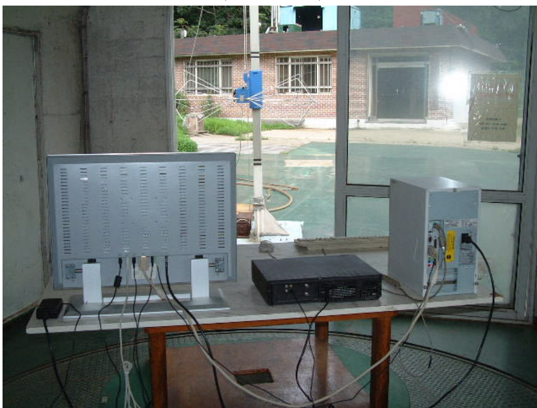
RADIATED EMISSION SETUP PHOTOGRAPH - REAR VIEW ( 30 - 300 MHz )
