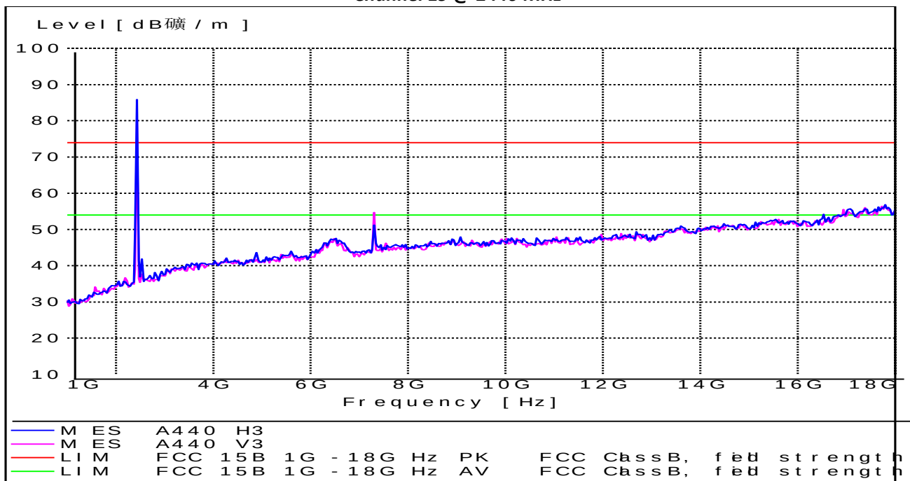
Channel 19 @ 2440 MHz
