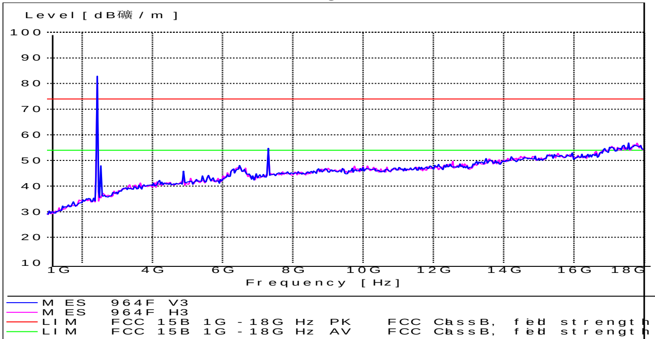
Channel 19 @ 2440 MHz
