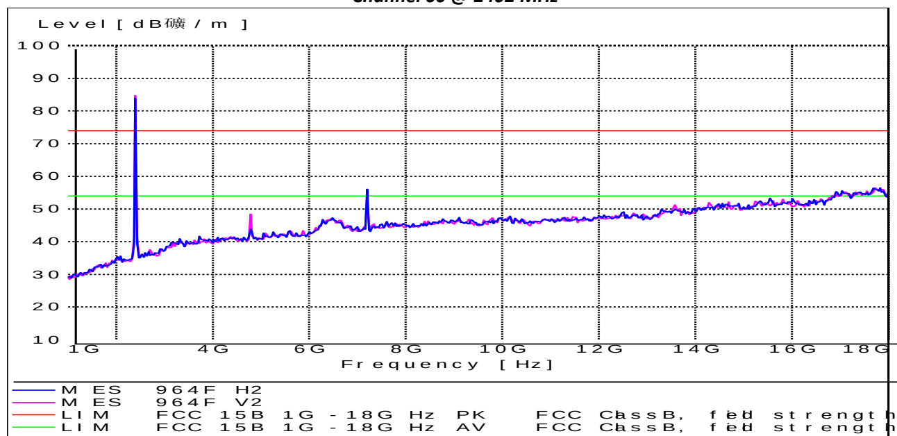
Channel 00 @ 2402 MHz
