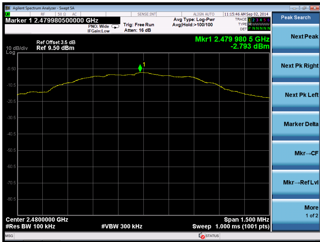
(Plot 6.4.1 C: Channel 39: 2480 MHz @ GFSK)
