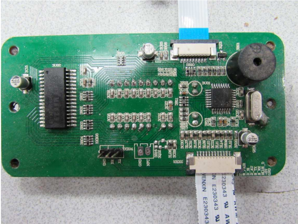
Back of display board
