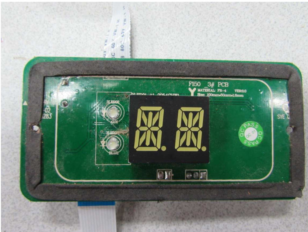
Front of display board
