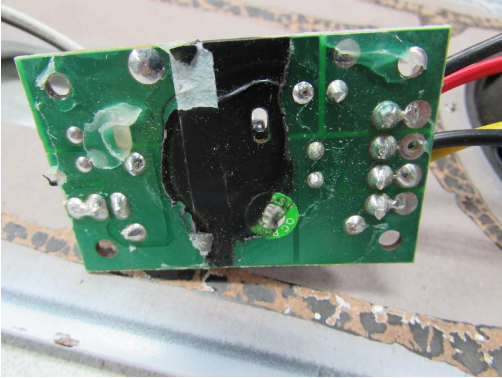
Back of audio board
