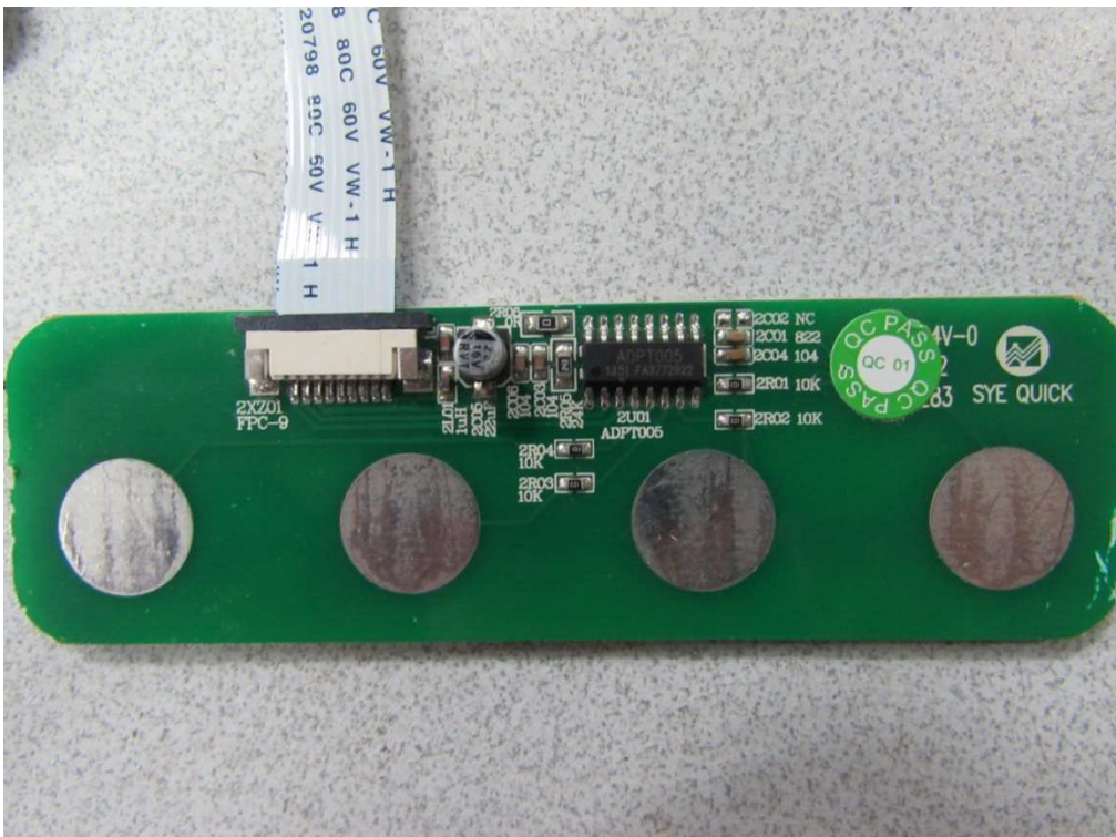
Front of touch board
