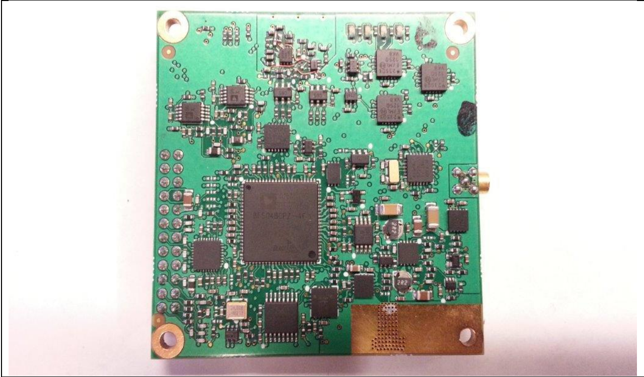
Photo: Xetawave XETA4 Transceiver Assembly Bottom
