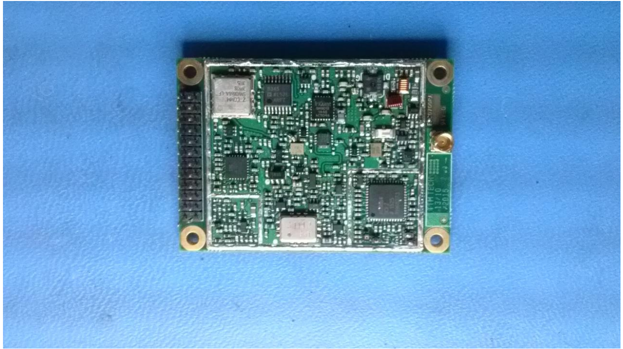
PHOTO: TOP SIDE XETA7M-T WITHOUT SHIELD
