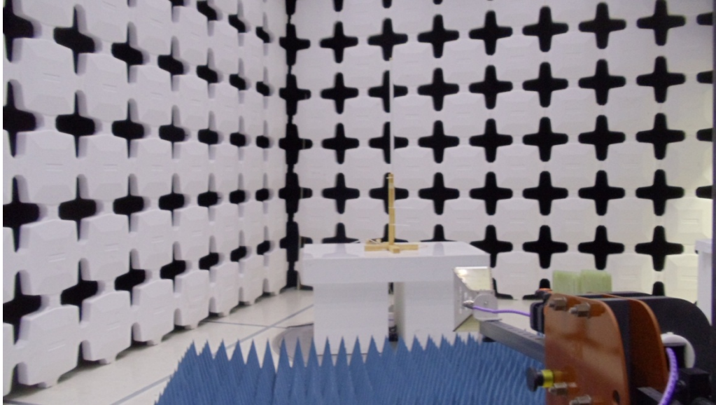
Test Setup for Radiated Emissions, 1GHz to 10GHz – Horizontal Polarization – Laird Antenna
