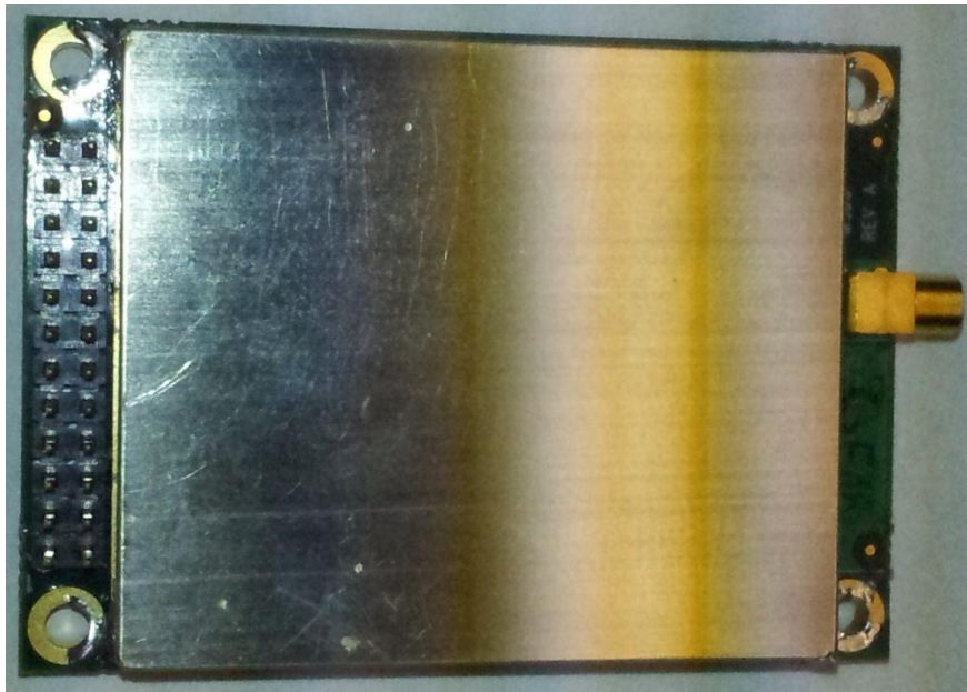
Photo: Xetawave MSD9 Transceiver Assembly Top with Shield
