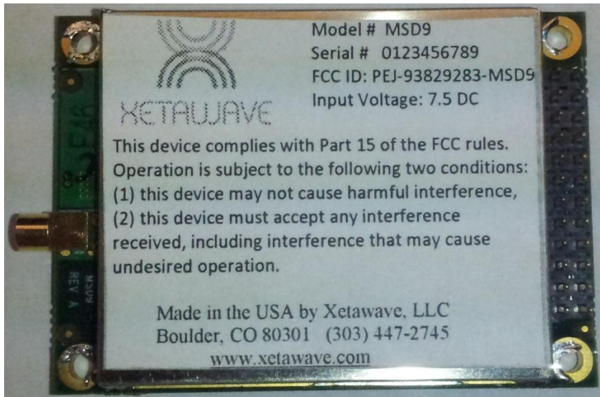
Photo: Xetawave MSD9 Transceiver Assembly Top with Label and Label Location
