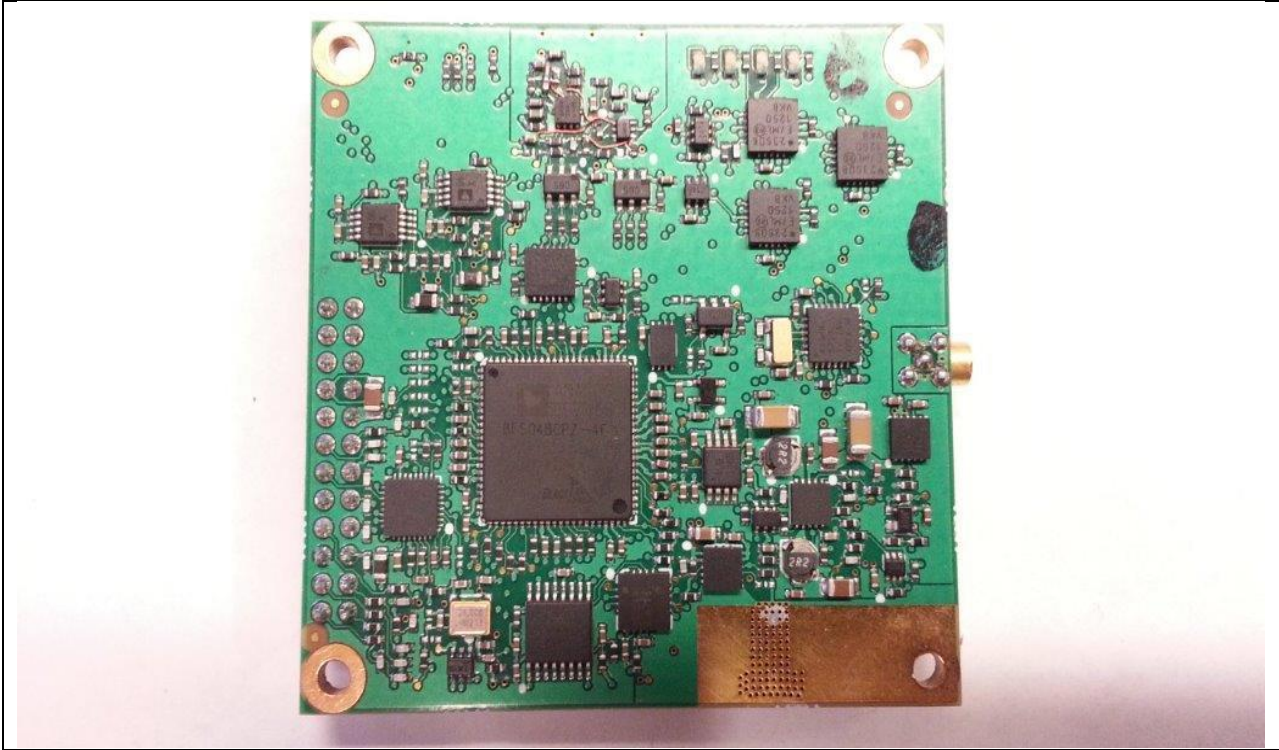
Xetawave XETA4m-HP Internal Photo: Transceiver Assembly Bottom
