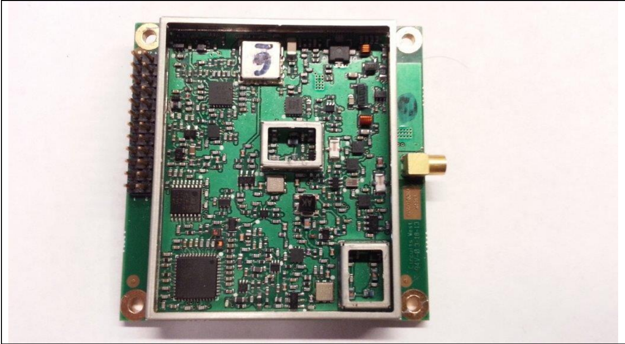
Xetawave XETA4m-HP Internal Photo: Transceiver Assembly Top without Shield
