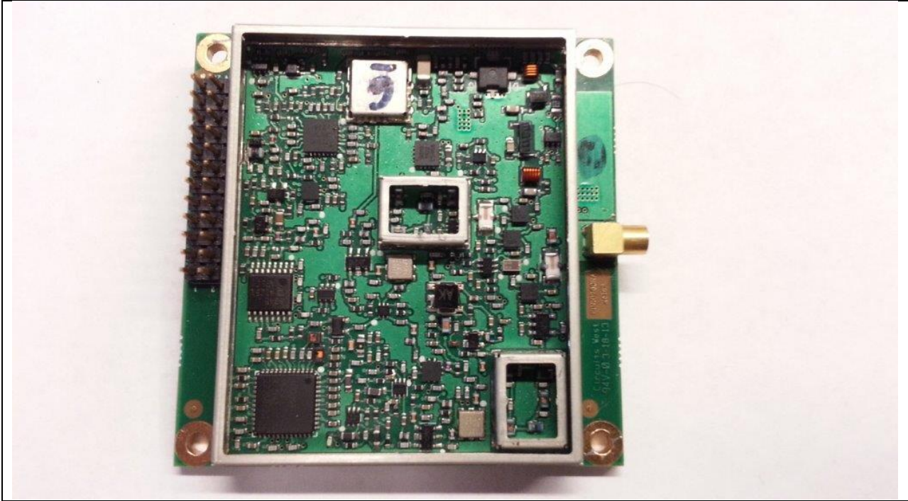
Photo: Xetawave XETA1 Transceiver Assembly Top without Shield
