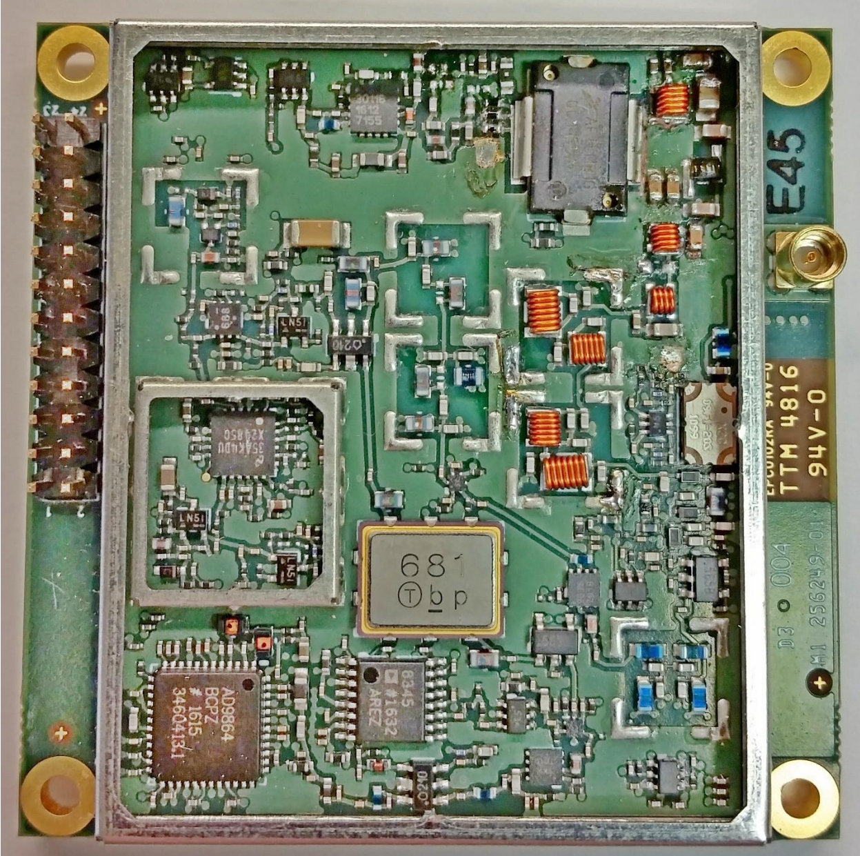
PHOTO: TOP SIDE XETA1-M2 WITHOUT SHIELD
