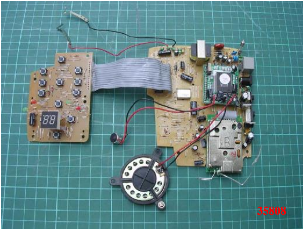
Photo 1: Internal photo of EUT (Base)
