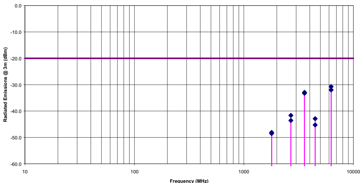
Radiated Emissions Measurements at 3 Meters OFTS SG-Sure Signal, Models Sure Signal, Sure Signal Max, Sure Signal CSR
