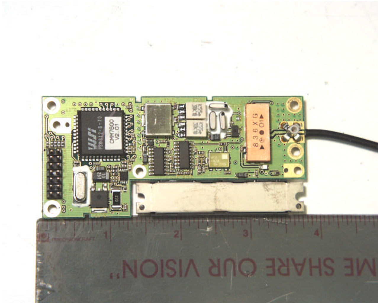
The STC Radio Transceiver Module, Model CU81KAB, FCC ID: APV0896
