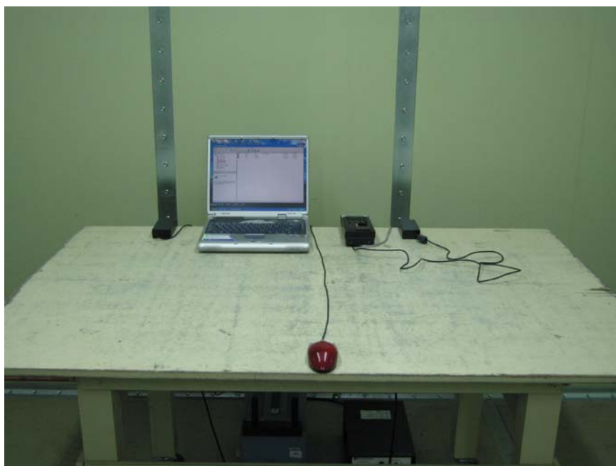
Photograph 2 : Setup for Conducted Emissions
