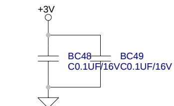
Bypass Capacitors for AP89341
