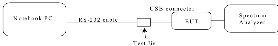
Figure 2: Emission bandwidth measurement configuration.
