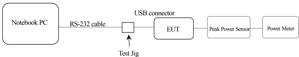
Figure 3: Output power measurement configuration.
