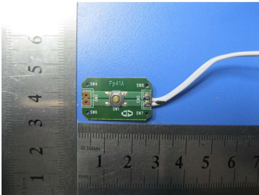
EUT –PCB Board Front View 1
