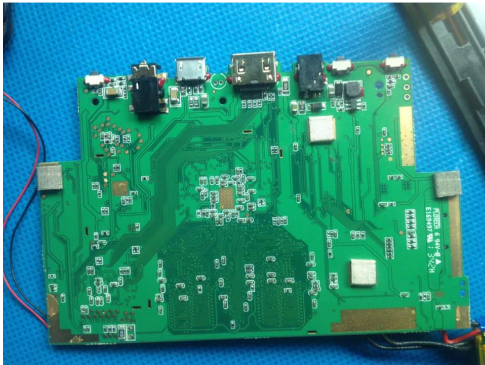
EUT – PCB View 5
