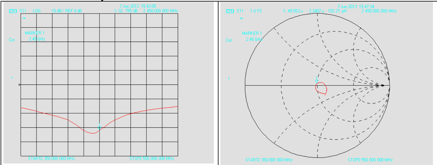
Dipole Verification plot: SID2450 2450MHz for Body:
