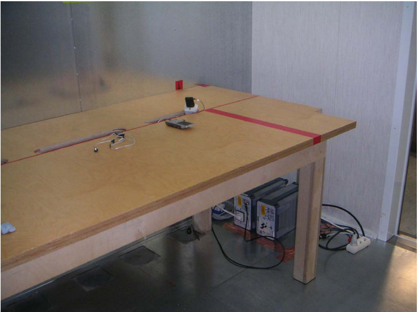
Picture 3 AC powerline conducted emission measurement BT TX/WLAN TX
