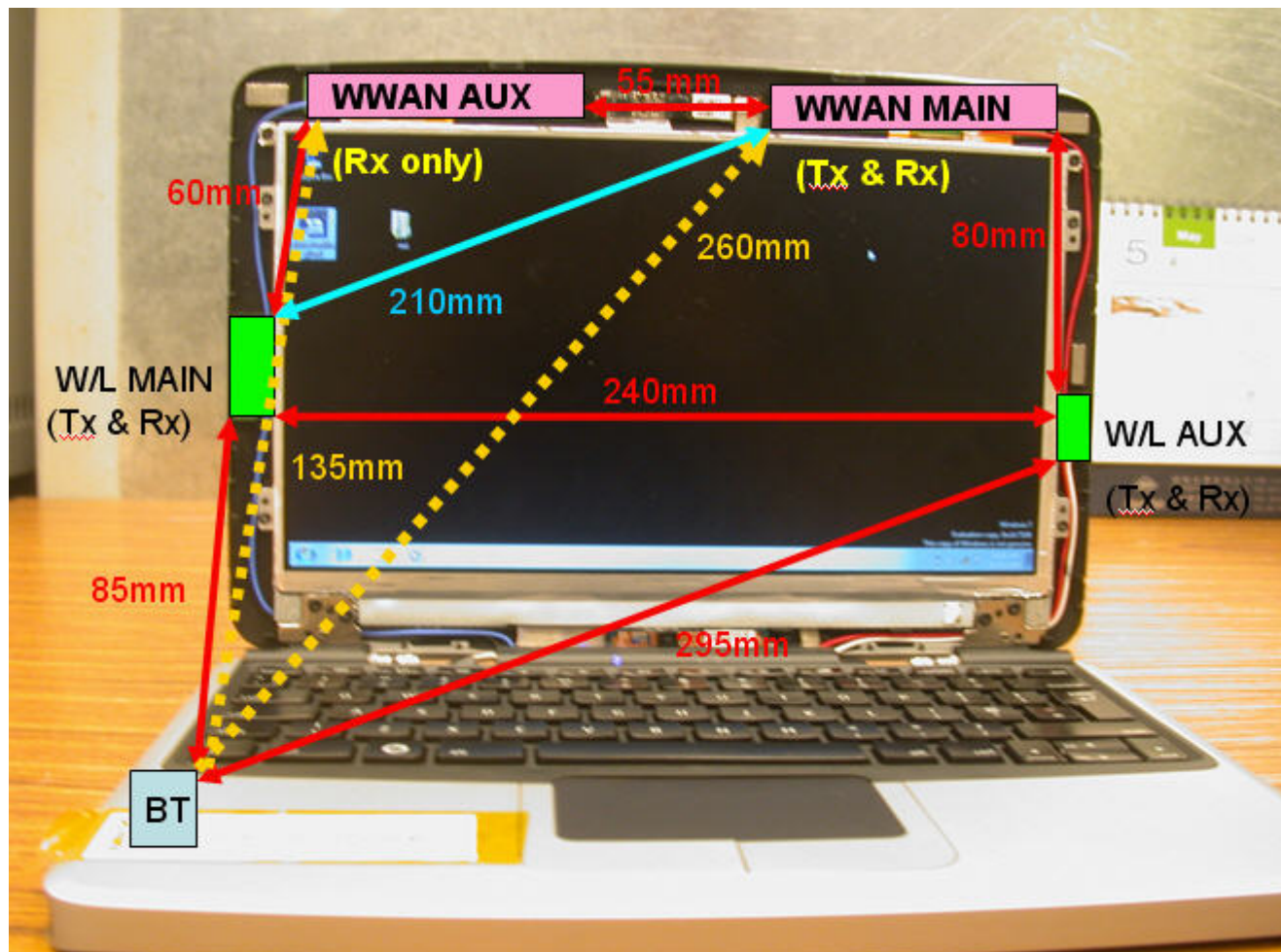
Picture 1. Antenna configuration
