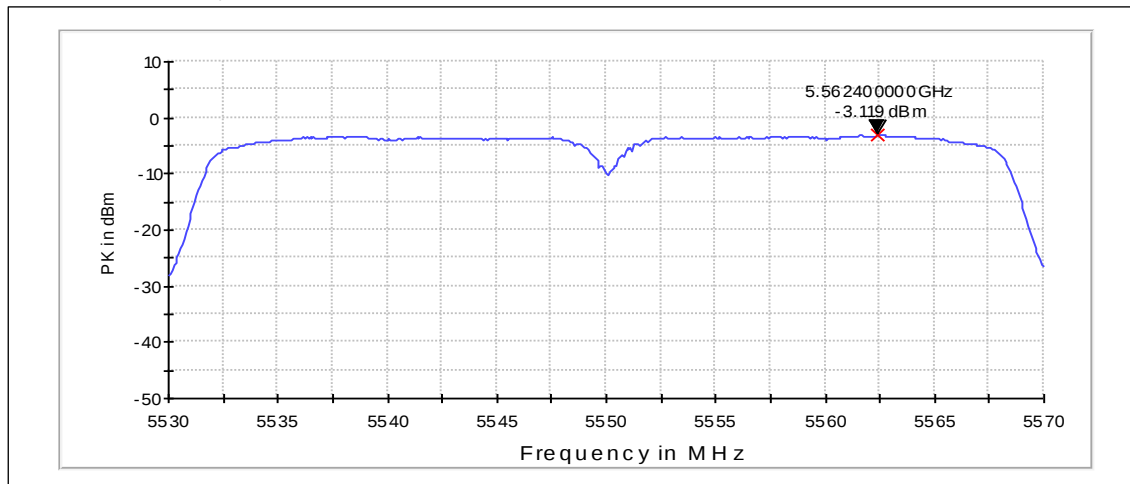
Channel 108+112 / 5550MHz
