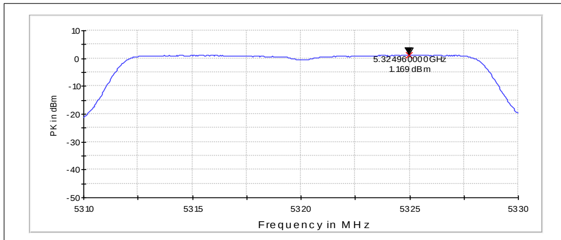
Channel 64 / 5320MHz
