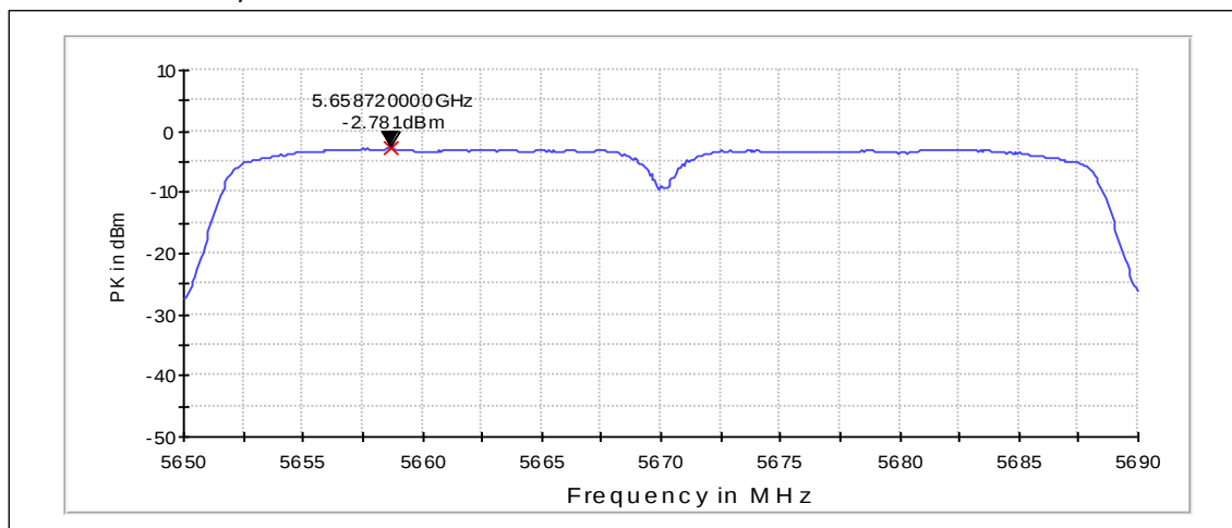
Channel 132+136 / 5670MHz
