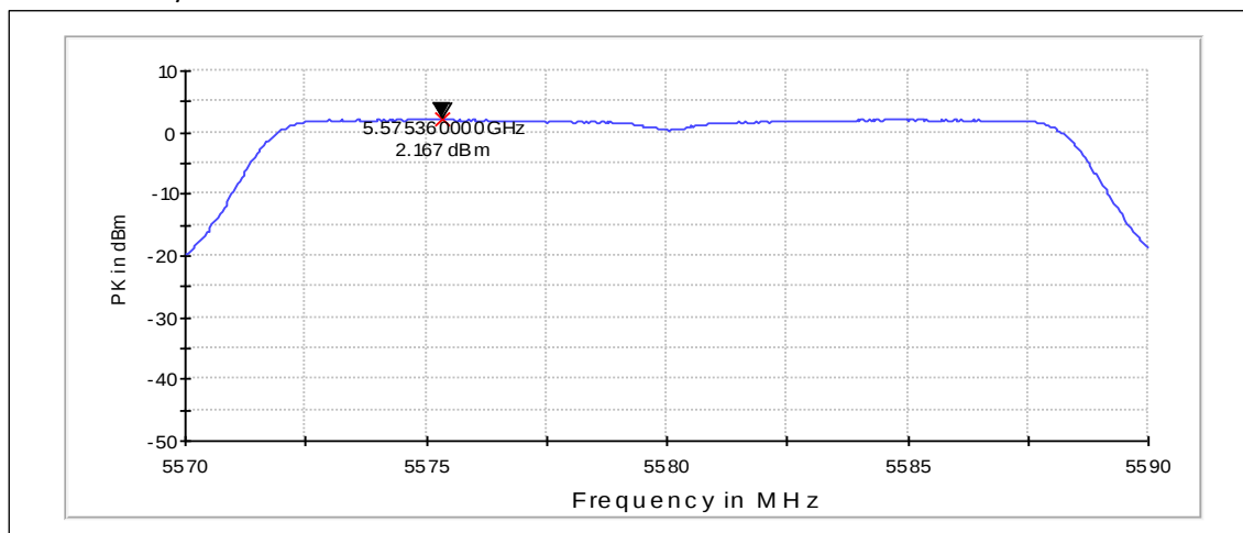
Channel 116 / 5580MHz
