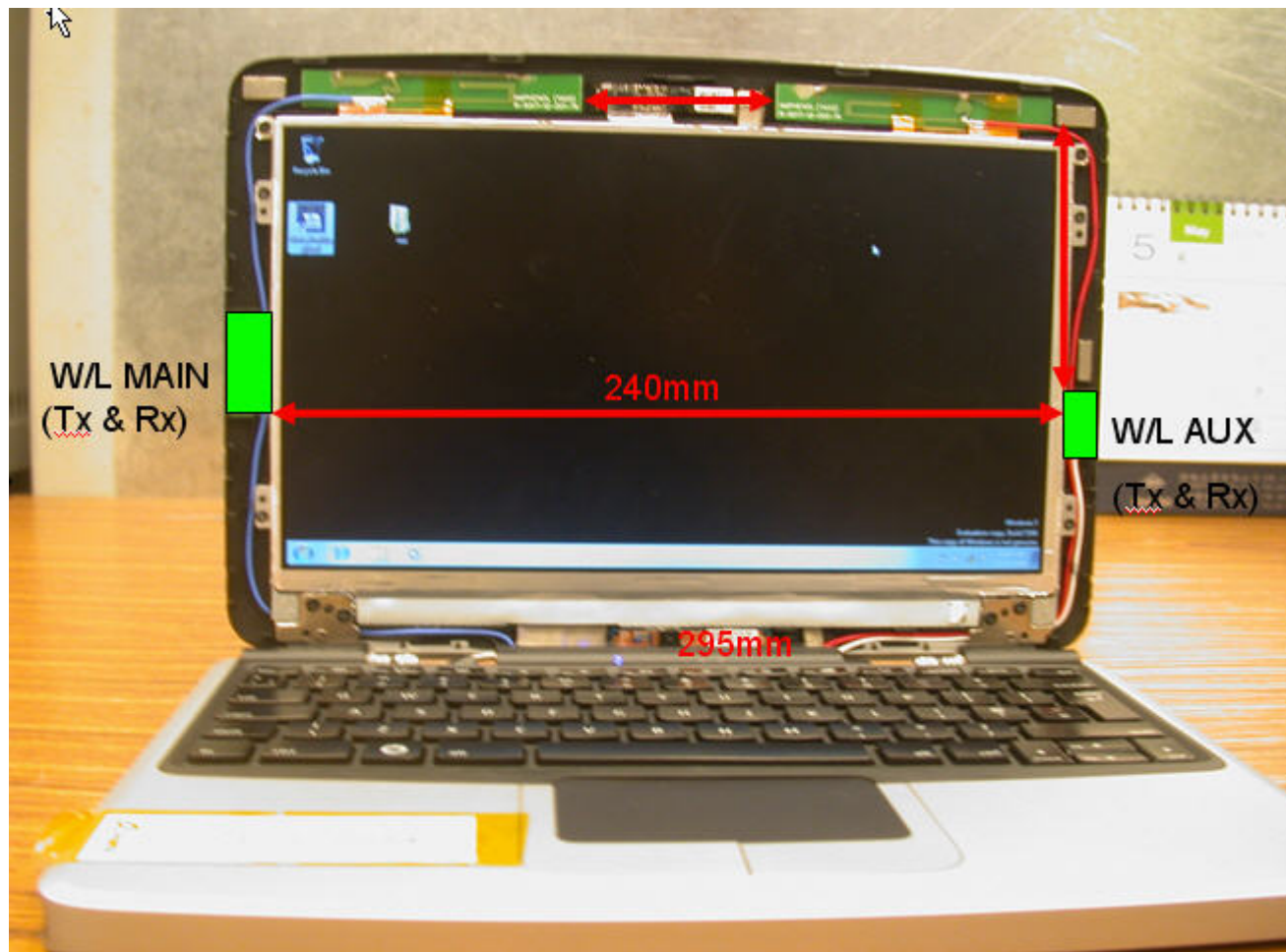
Picture 1. Antenna configuration
