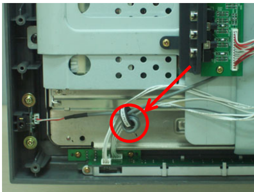
Ferrite Cores are inserted additionally.
