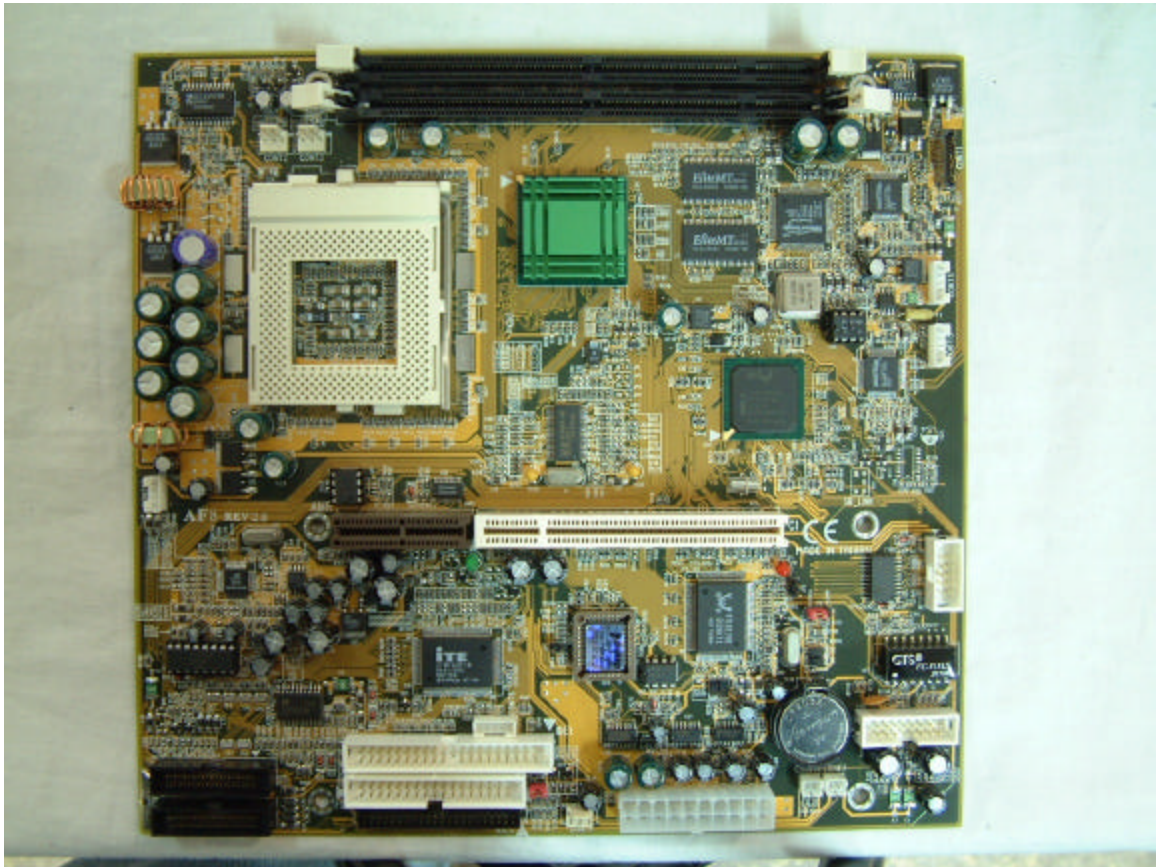
Main Board Component Side
