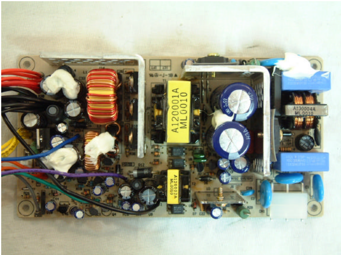
Power supply component side
