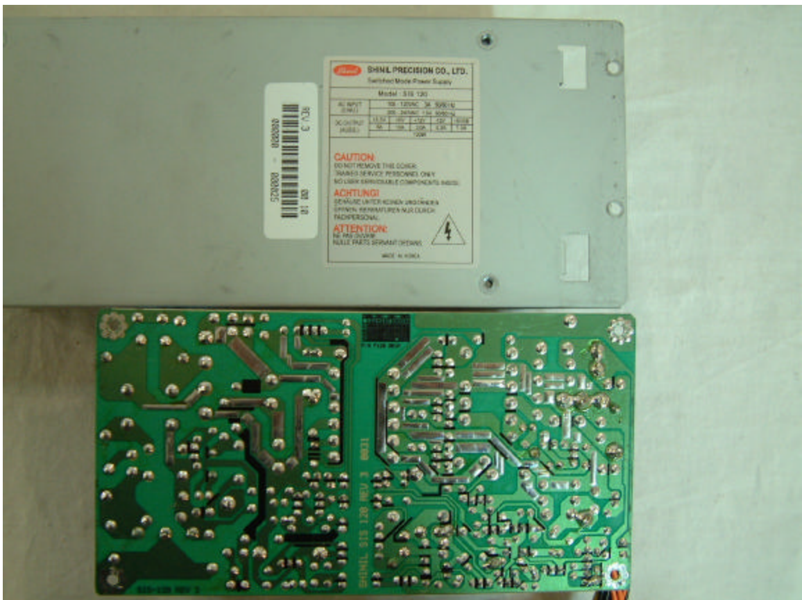
Power supply solder side
