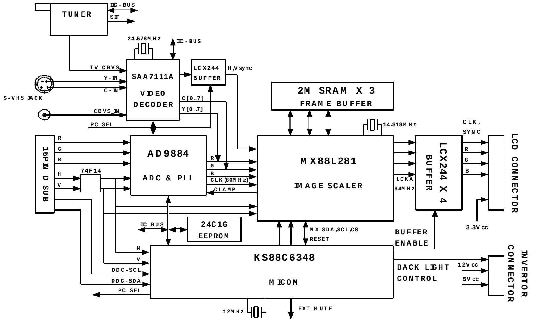
TFT LCD TV Block Diagram
