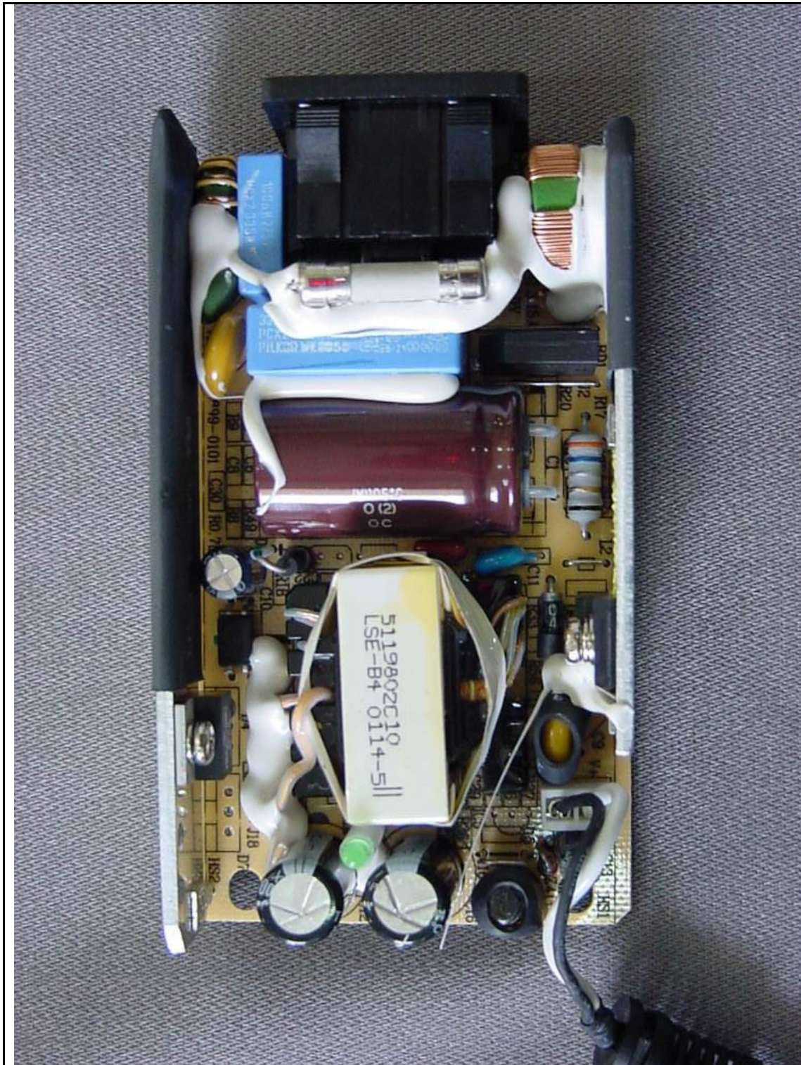
[ Top View of the AC/DC Adaptor Board ]
