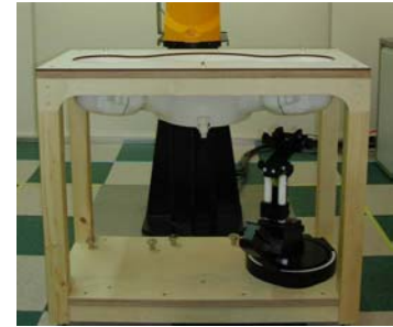
Figure 8. SAM Phantom
