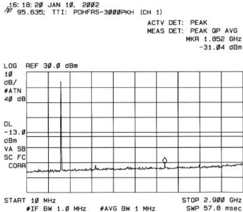
CHANNEL 1 OUT OF BAND 10 - 2900 MHz
