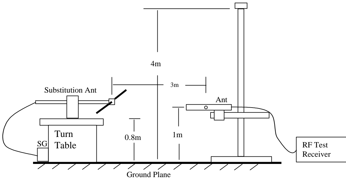
Fig 3: Radiated Emission – Substitution Method below 1000 MHz
