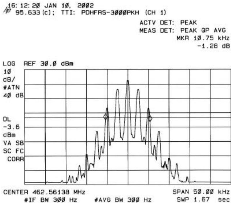
CHANNEL 1 OCCUPIED BANDWIDTH
