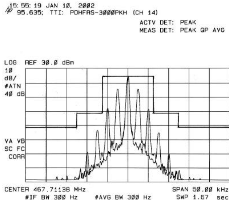
CHANNEL 14 EMISSION MASK
