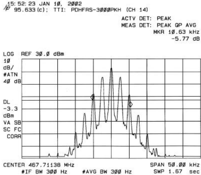
CHANNEL 14 OCCUPIED BANDWIDTH
