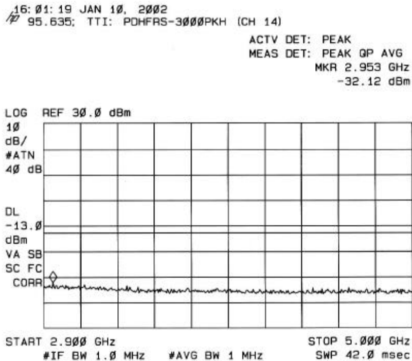
CHANNEL 14 OUT OF BAND 2.9 – 5 GHz
