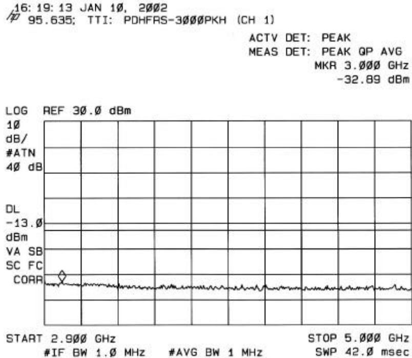
CHANNEL 1 OUT OF BAND 2.9 – 5 GHz
