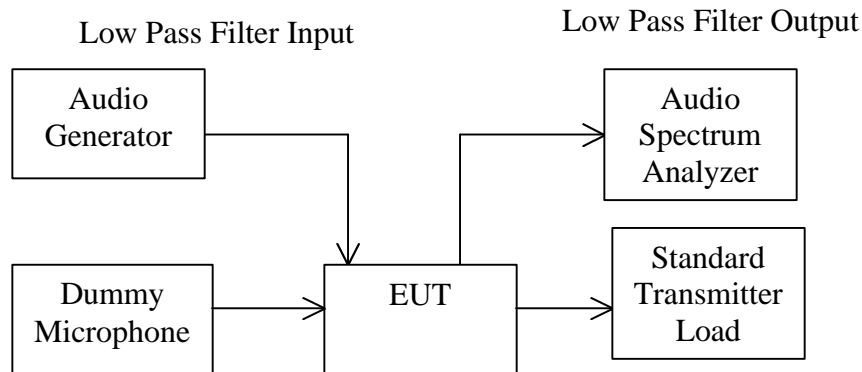
Figure 5: Audio low pass filter response measurement configuration
