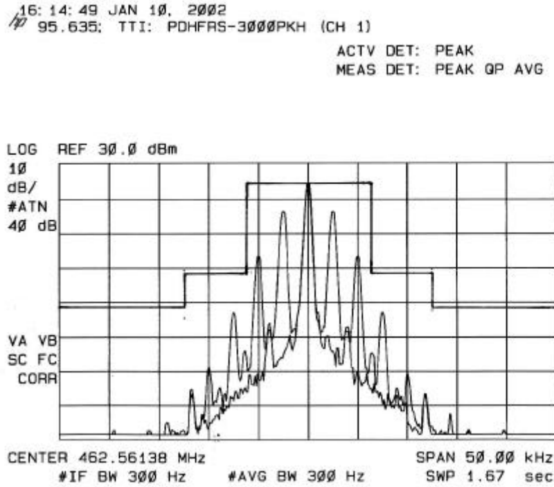
CHANNEL 1 EMISSION MASK
