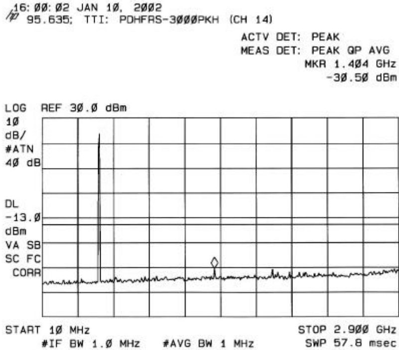
CHANNEL 14 OUT OF BAND 10 – 2900 MHz
