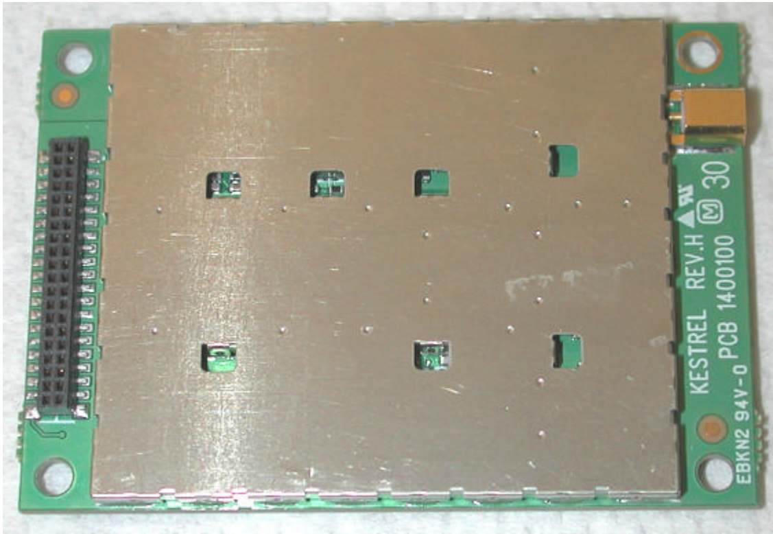
#3. SB555 Radio side with shield on.
