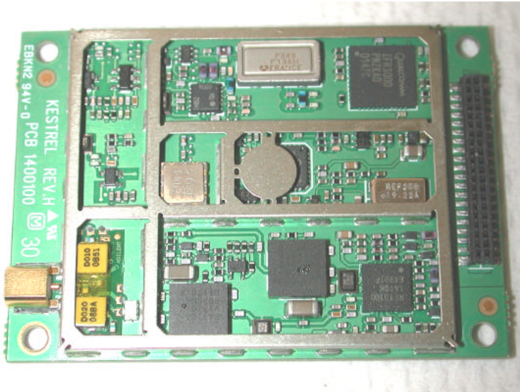
#4. SB555-T Radio side with shield off.
