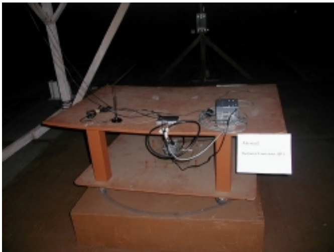
Rear View Maximized Radiated Emissions
