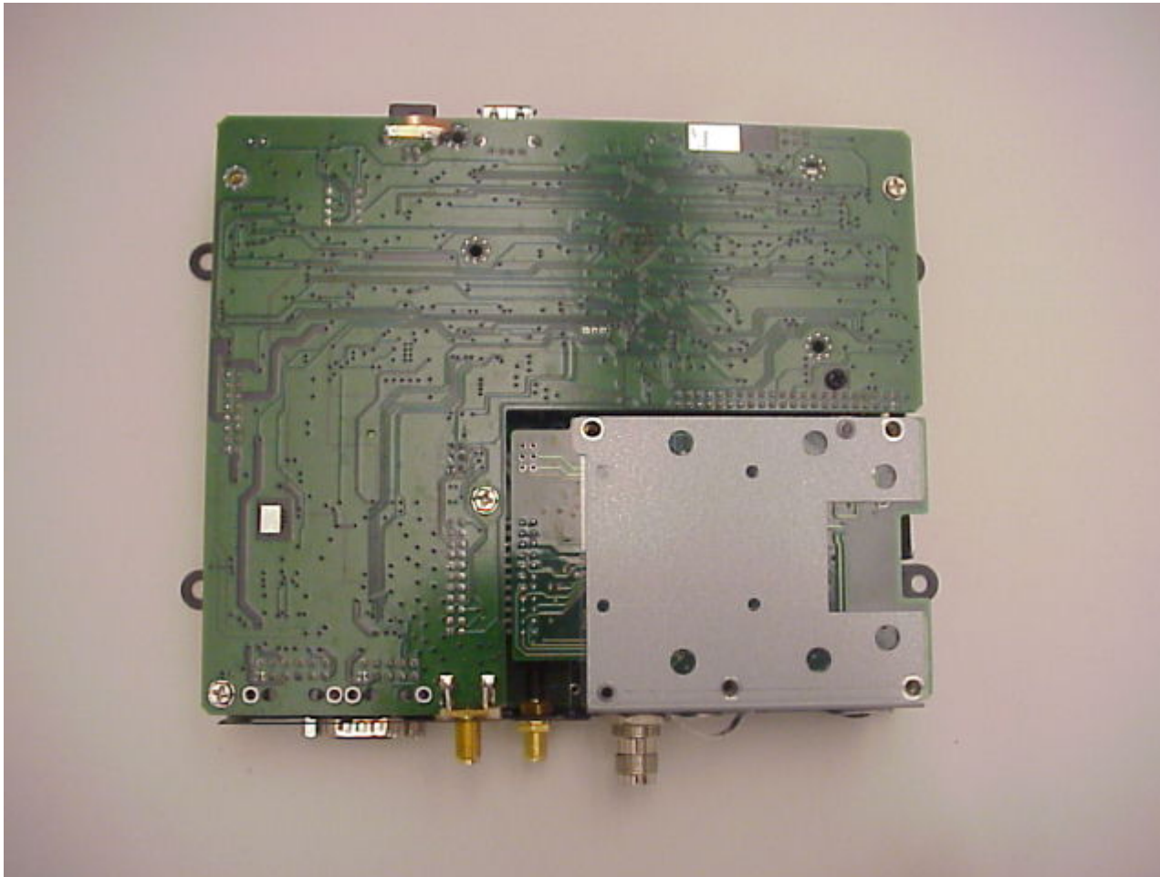
EUT – TOP OPEN VIEW 1
