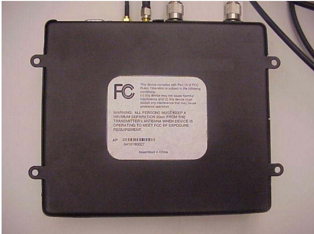
iWM3140 – BOTTOM VIEW
