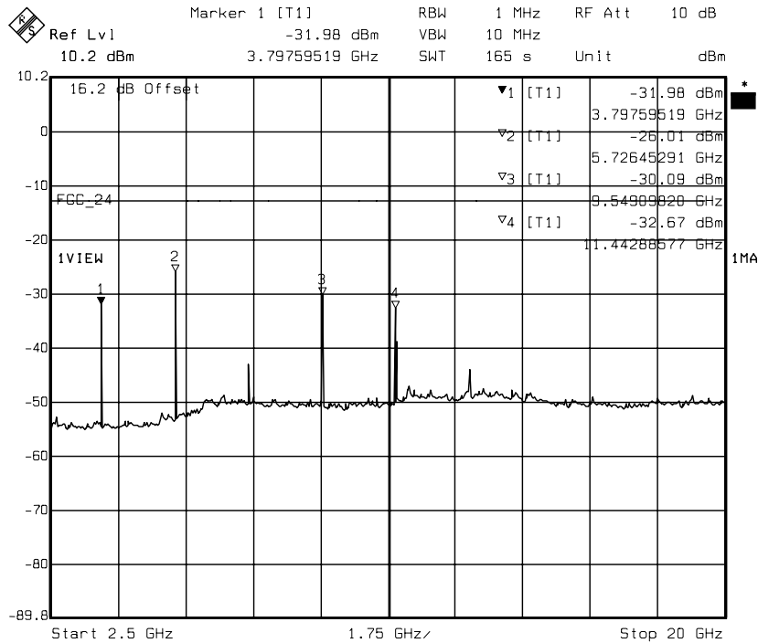
diagram 14.12: carrier on channel 810 (1909.8 MHz)
