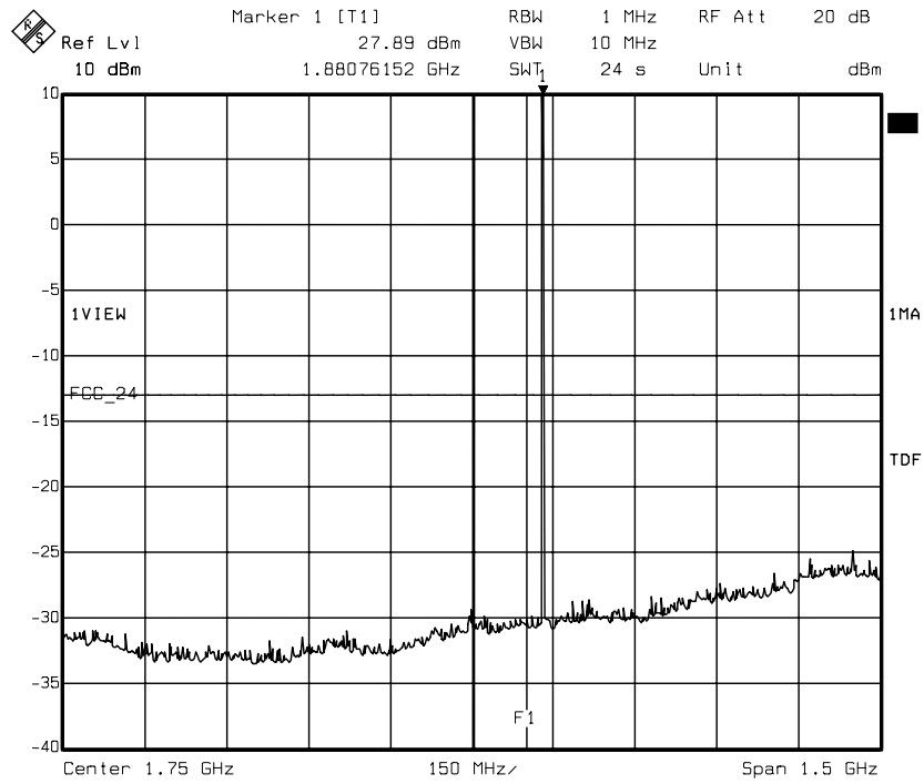
diagram 8.07: carrier on channel 661 (1880 MHz), TCH mode
