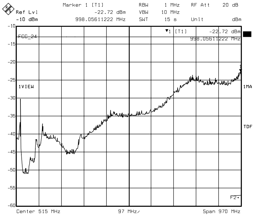
Title: FCC24 Messung, Emission Sweep 2 Date: 22.JUL.2002 21:38:01
