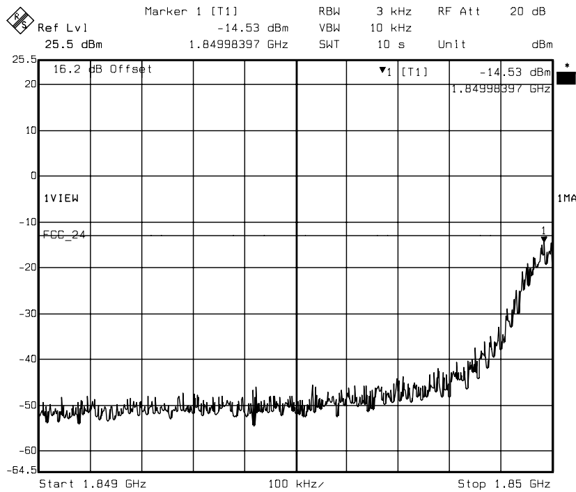
diagram 14.04: carrier on channel 512 (1850,2 MHz)
