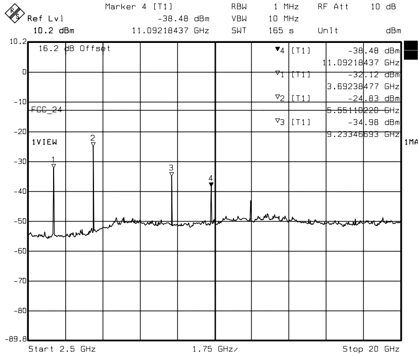
diagram 14.03: carrier on channel 512 (1850,2 MHz)
