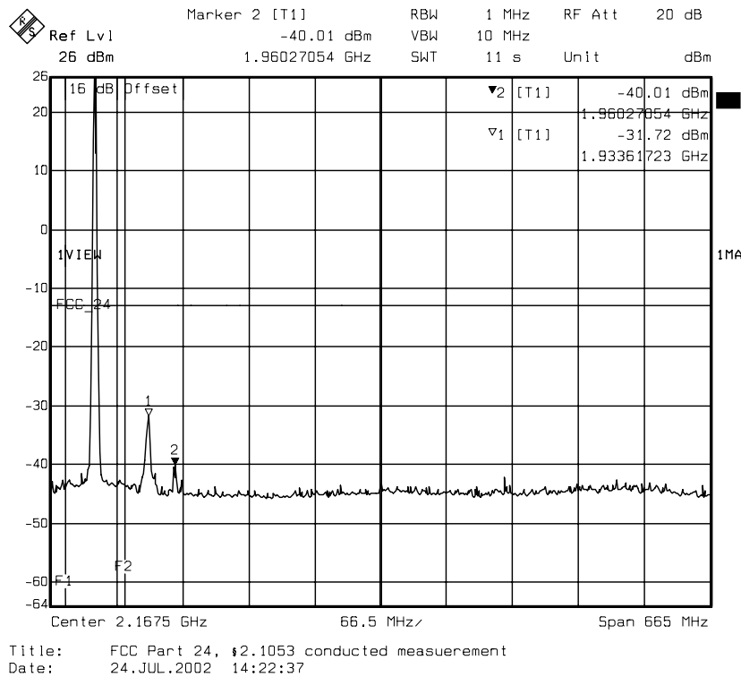
diagram 14.06: carrier on channel 661 (1880 MHz)
