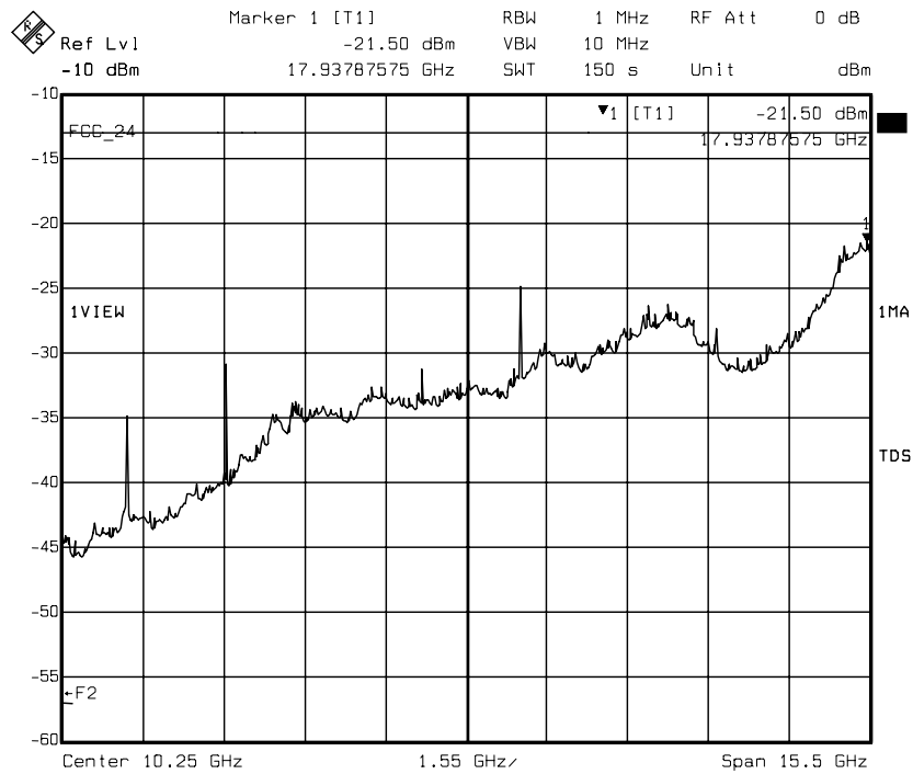
diagram 8.08: carrier on channel 661 (1880 MHz), TCH mode
