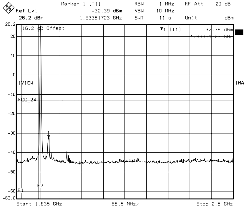
diagram 14.11: carrier on channel 810 (1909.8 MHz)
