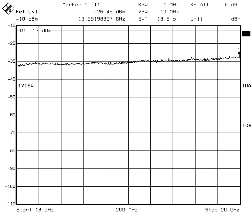
Title: FCC Sweep 8 horizontal channel 512 Date: 30.JUL.2002 13:21:06
