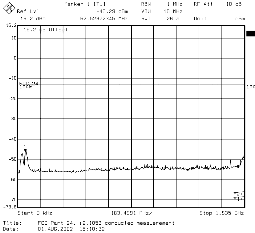
diagram 14.05: carrier on channel 661 (1880 MHz)
