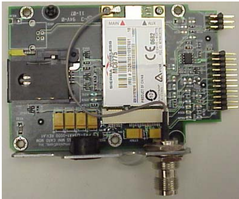
MC8775 MODULE CLOSE-UP VIEW
