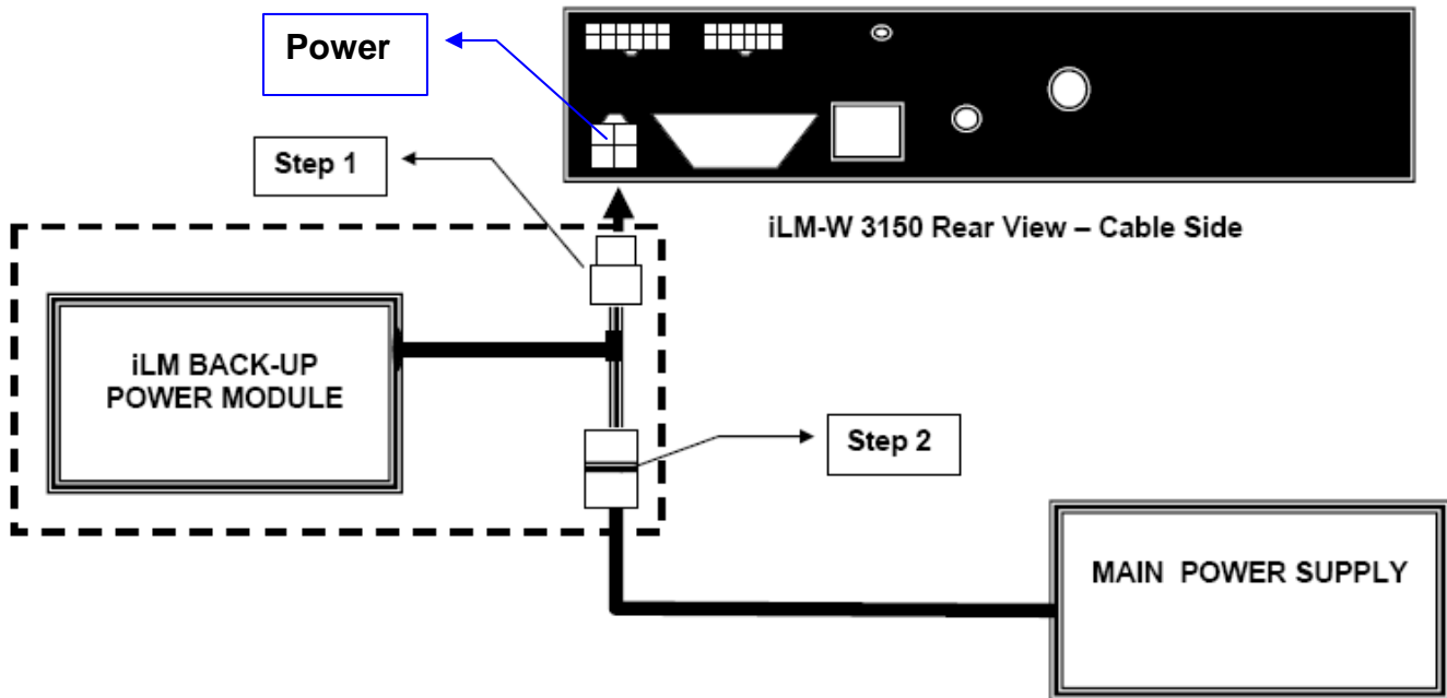
iLM BACK-UP POWER MODULE AND iLM-W 3150 WIRING DIAGRAM
